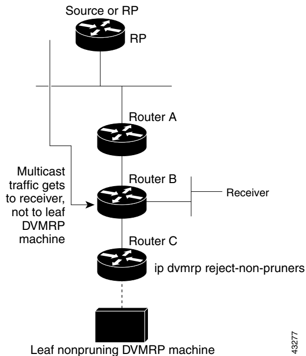
Figure 2 Router Rejects Nonpruning DVMRP Neighbor
