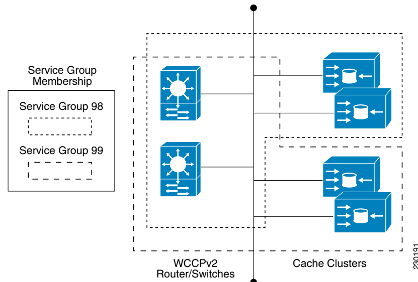
Figure 3 WCCP Service Groups
