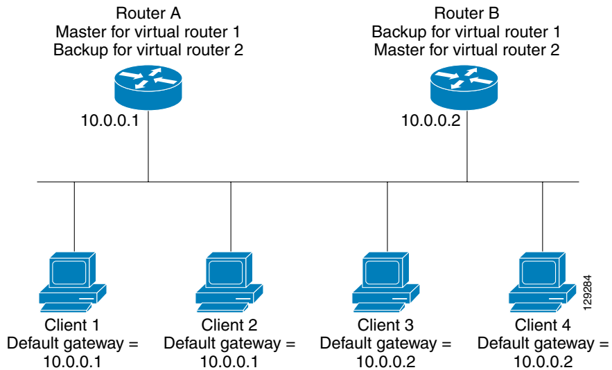
Figure 2 Load Sharing and Redundancy VRRP Topology
