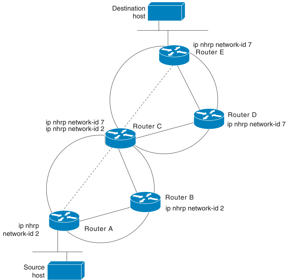
Figure 2 Two Logical NBMA Networks over One Physical NBMA Network
