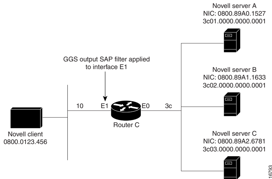
Figure 6 GGG SAP Response Filter
