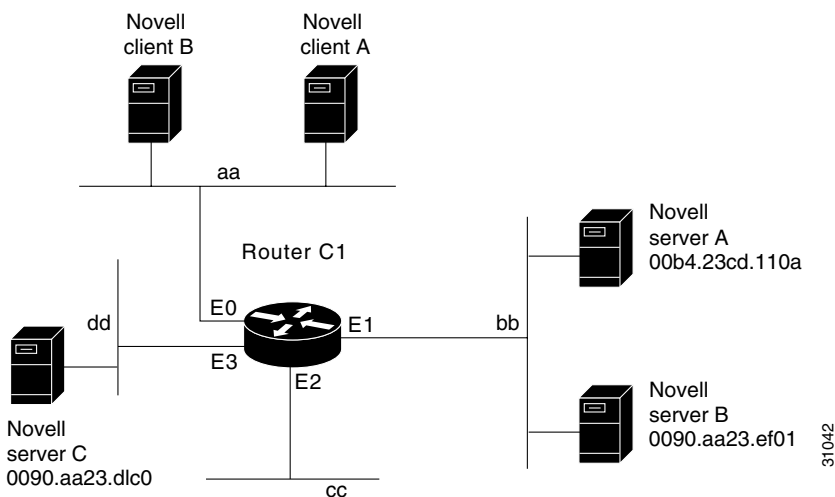
Figure 7 IPX Clients Requiring Server Access Through a Router
