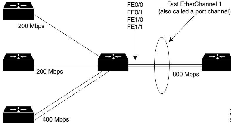
Figure 2 Fast Ethernet Interfaces Aggregated into a Fast EtherChannel
