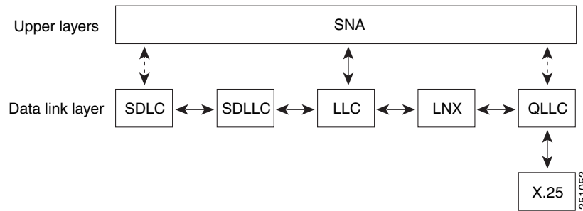
Figure 2 SNA Data Link Layer Support
