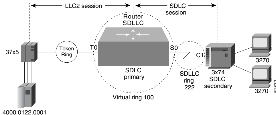
Figure 9 SDLLC Communication Between a 37x5 and a 3x74 Connected to the Same Router (Direct Connection)
