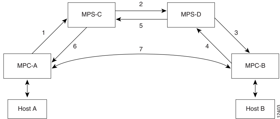
Figure 23 MPOA Message Flow Between MPCs and MPSs
