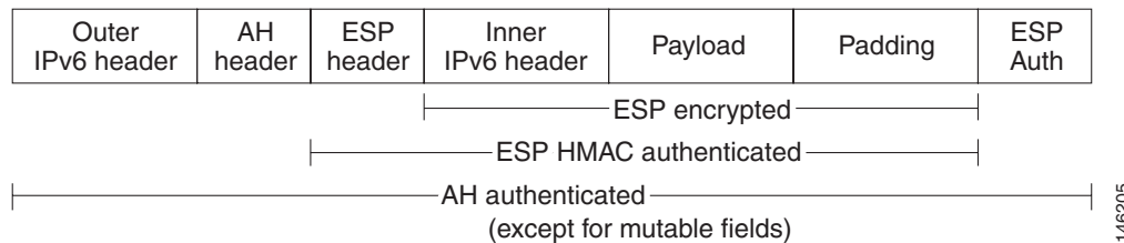
Figure 23 IPv6 IPsec Packet Format
