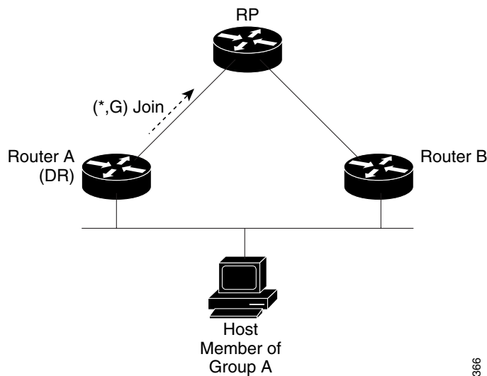
Figure 31 Designated Router Election on a Multiaccess Segment
