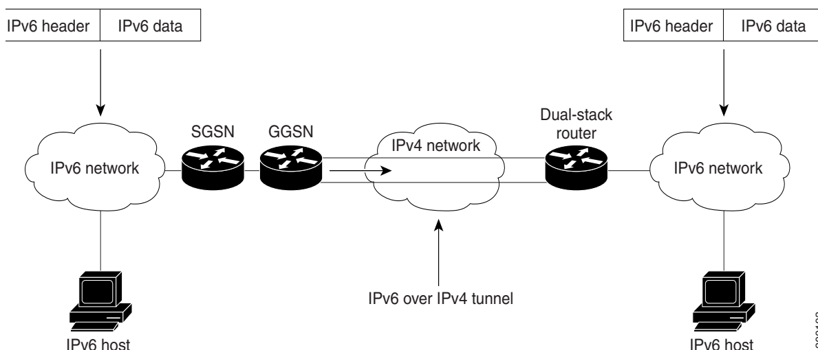
Figure 5-1 IPv6 over IPv4 Tunnel Configuration
