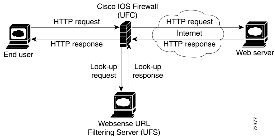
Figure 1 Firewall WEBSense URL Filtering Sample Topology
