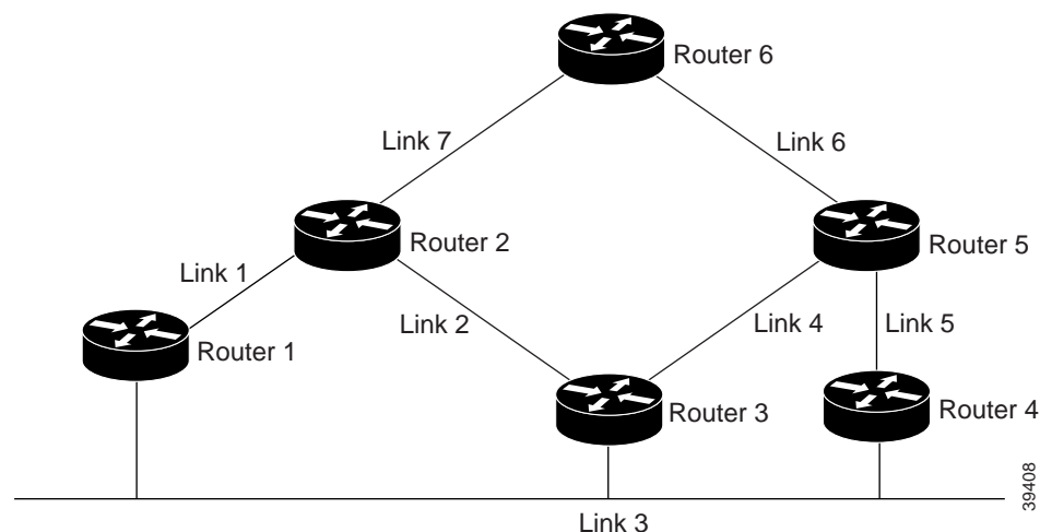
Figure 4 Sample Network for Transitioning from TDP to LDP
