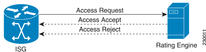
Figure 11 Quota Reauthorization Access-Request
