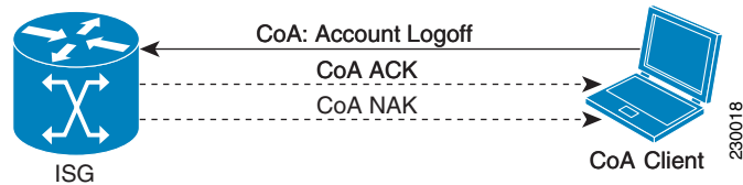
Figure 7 CoA-Request; Account Logoff
