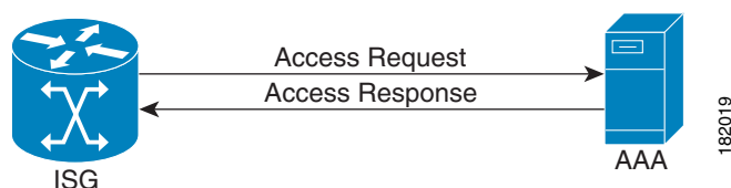
Figure 10 Accounting Request/Response
