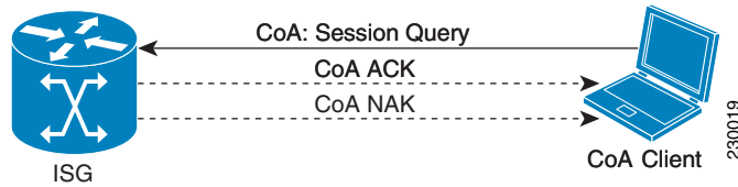
Figure 8 CoA-Request, Session Query
