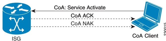
Figure 3 CoA-Request; Service Activate
