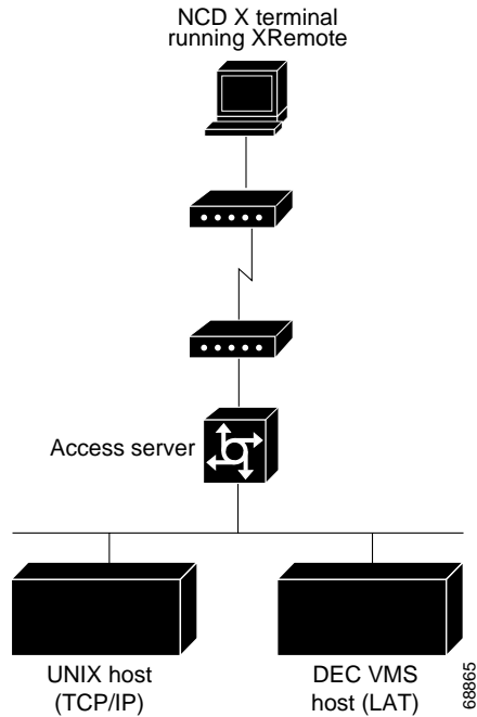
Figure 5 XRemote Connection
