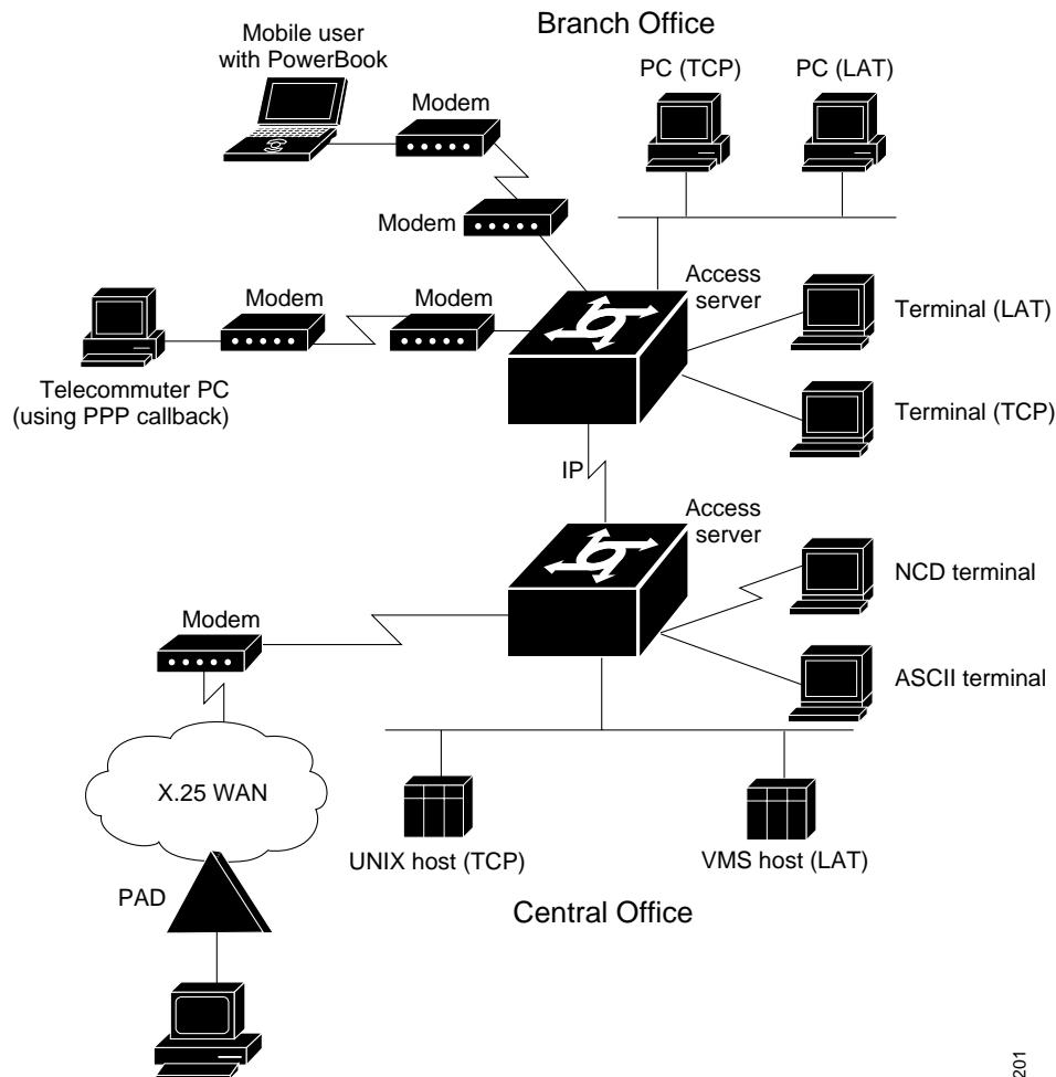
Figure 2 Access Service Functions
