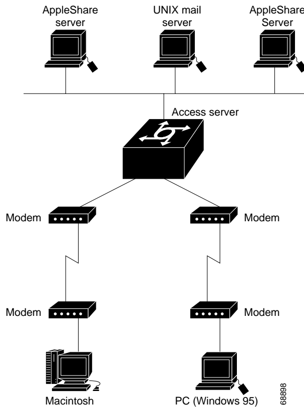
Figure 4 Remote Node Connection—Macintosh and PC Users Dialing In
