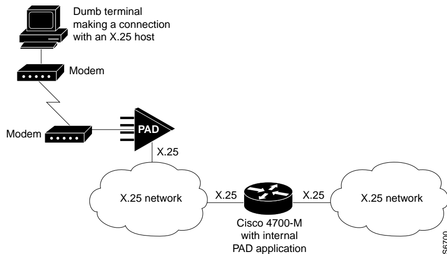
Figure 3 Standard X.25 Dial-Up Connection
