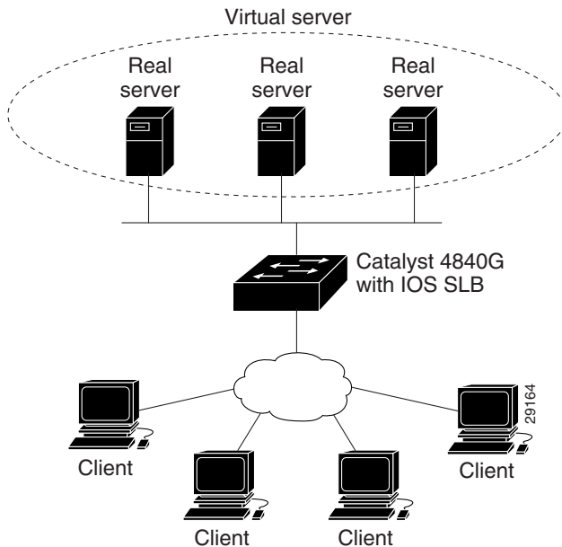
Figure 23 Logical View of IOS SLB
