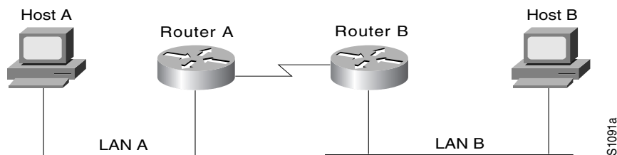
Figure 18 Network Demonstrating Output Address List Filtering
