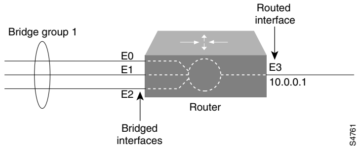
Figure 7 Integrated Routing and Bridging Interconnecting a Bridged Network with a Routed Network
