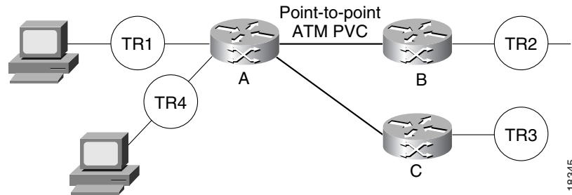
Figure 50 Multiple ATM PVCs and Multiple Virtual Rings on a Router
