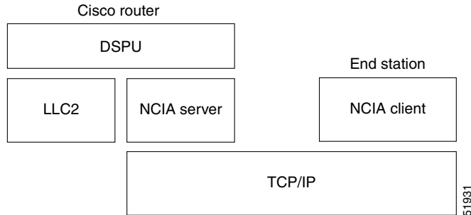
Figure 207 Logical View of NCIA Server with DSPU
