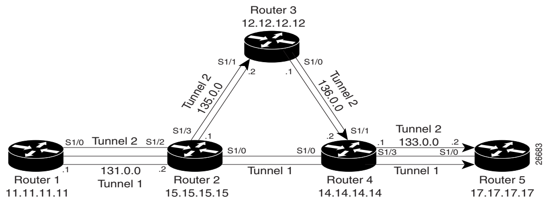
Figure 3 Sample MPLS Traffic Engineering Tunnel Configuration
