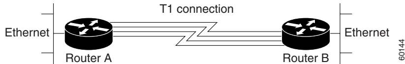
Figure 48 Inverse Multiplexing Application Using Multilink PPP
