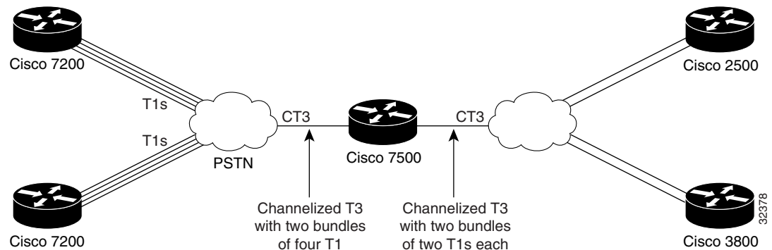
Figure 47 Diagram of a Typical VIP MLP Topology
