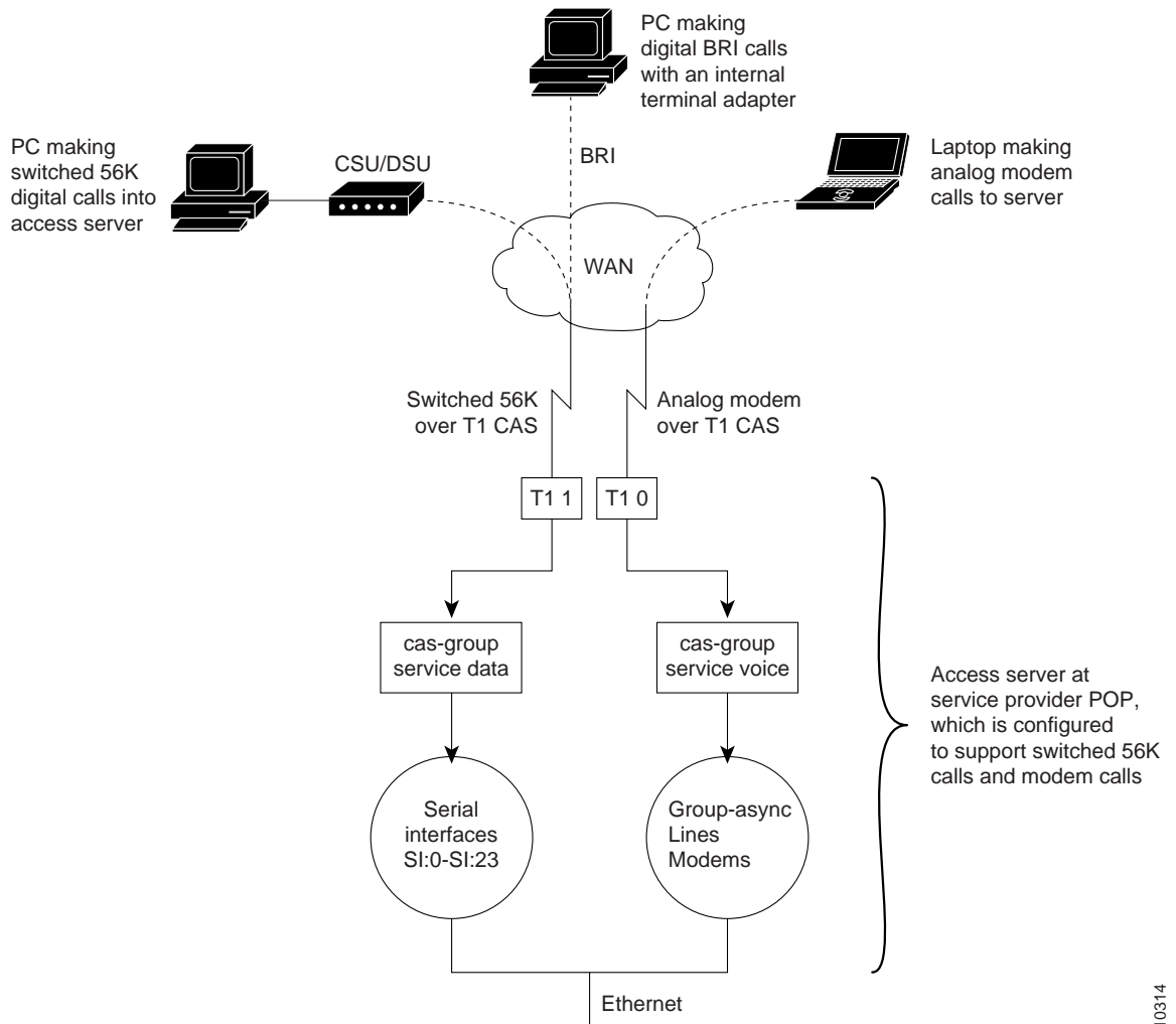
Figure 39 Processing Components for Switched 56K Calls Versus Analog Modem Calls
