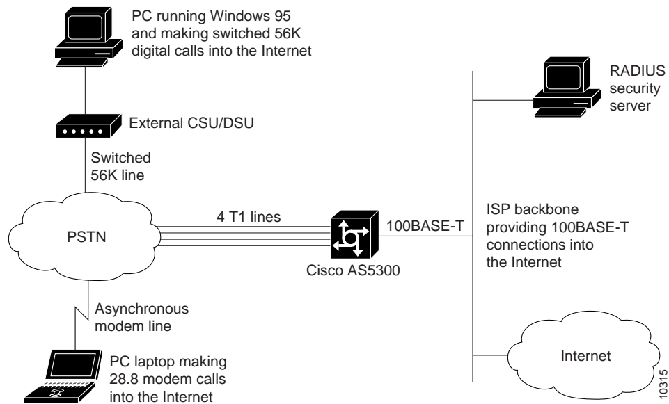
Figure 41 PCs Making Switched 56K and Analog Modem Calls into a Cisco AS5300 Access Server
