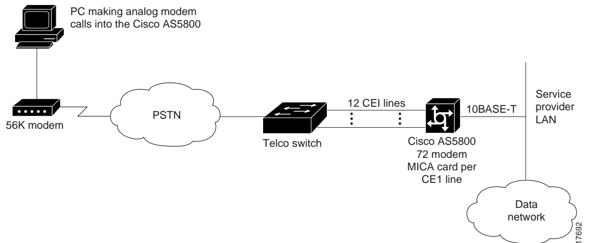
Figure 44 Service Provider Using E1 R1 Modified Signaling with a Cisco AS5800 Access Server
