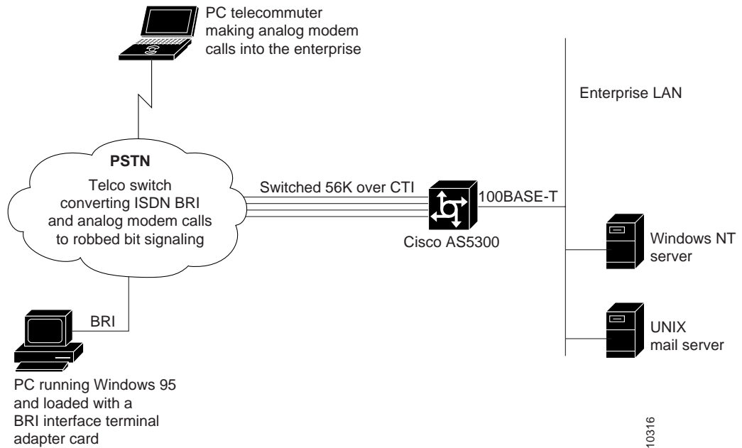
Figure 40 Remote PC Making BRI Digital Calls via Switched 56K to a Cisco AS5300 Access Server
