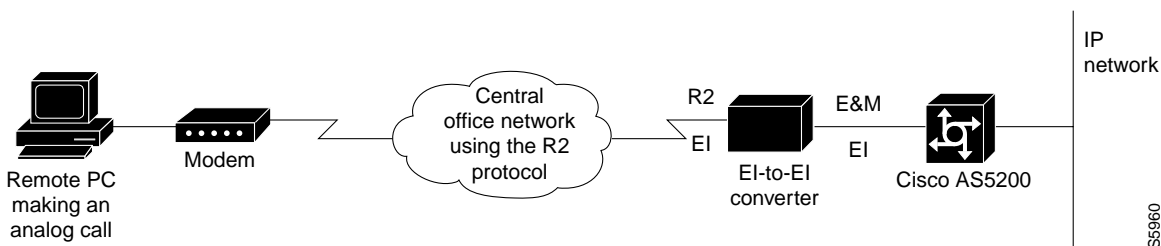
Figure 37 Remote PC Accessing Network Resources Through the Cisco AS5200 Access Server
