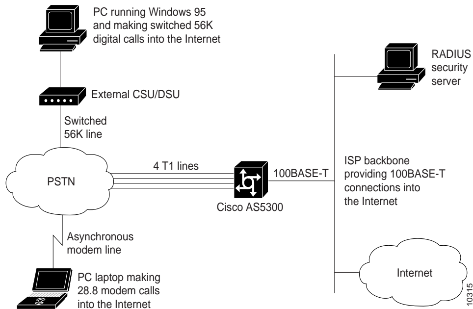
Figure 38 PCs Making Switched 56K and Analog Modem Calls into a Cisco AS5300 Access Server
