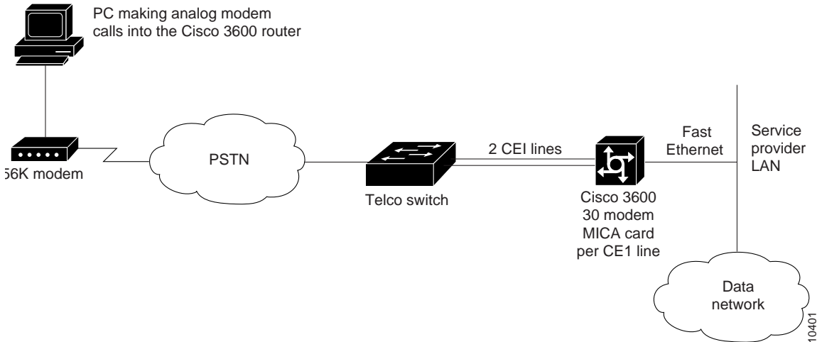
Figure 42 Service Provider Using E1 R2 Signaling and a Cisco AS3640 Router
