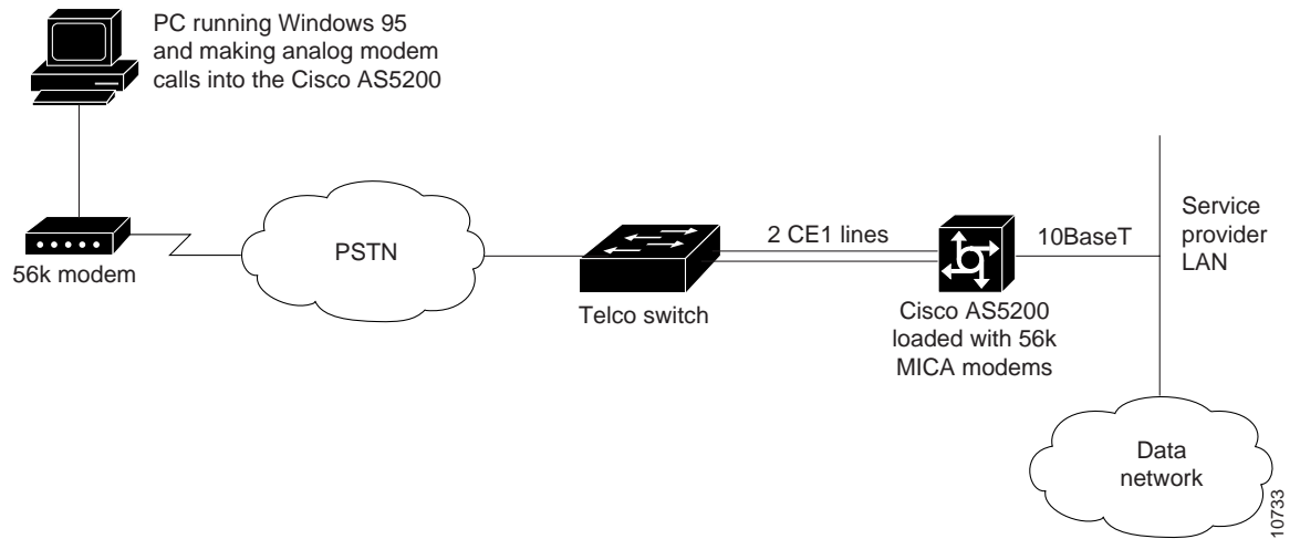
Figure 43 Service Provider Using E1 R1 Signaling with a Cisco AS5200 Access Server
