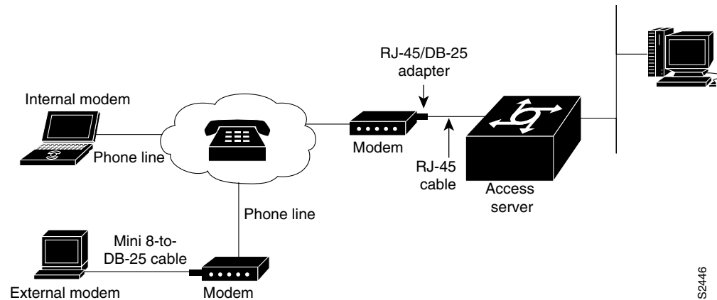
Figure 108 ARA Server Cabling and Connections
