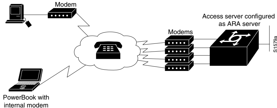
Figure 107 ARA Configuration Overview
