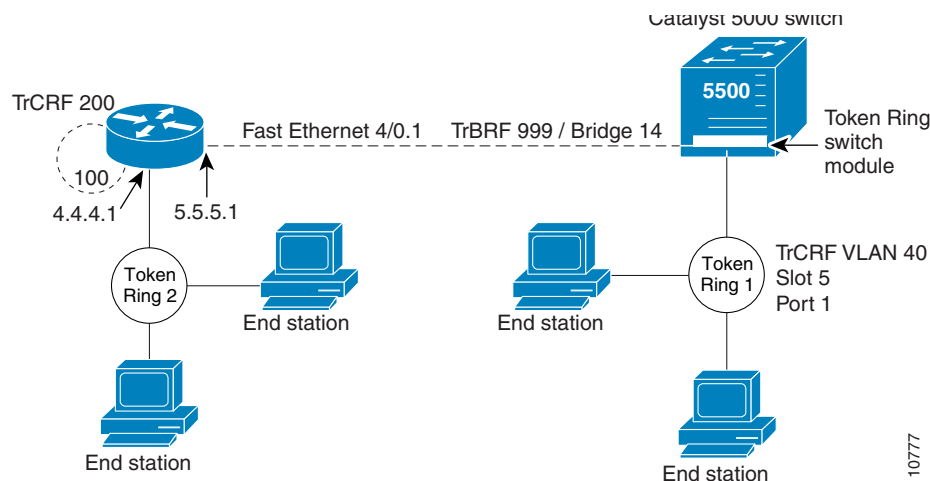
Figure 44 Routing with RIF Between a TRISL VLAN and a Token Ring Interface
