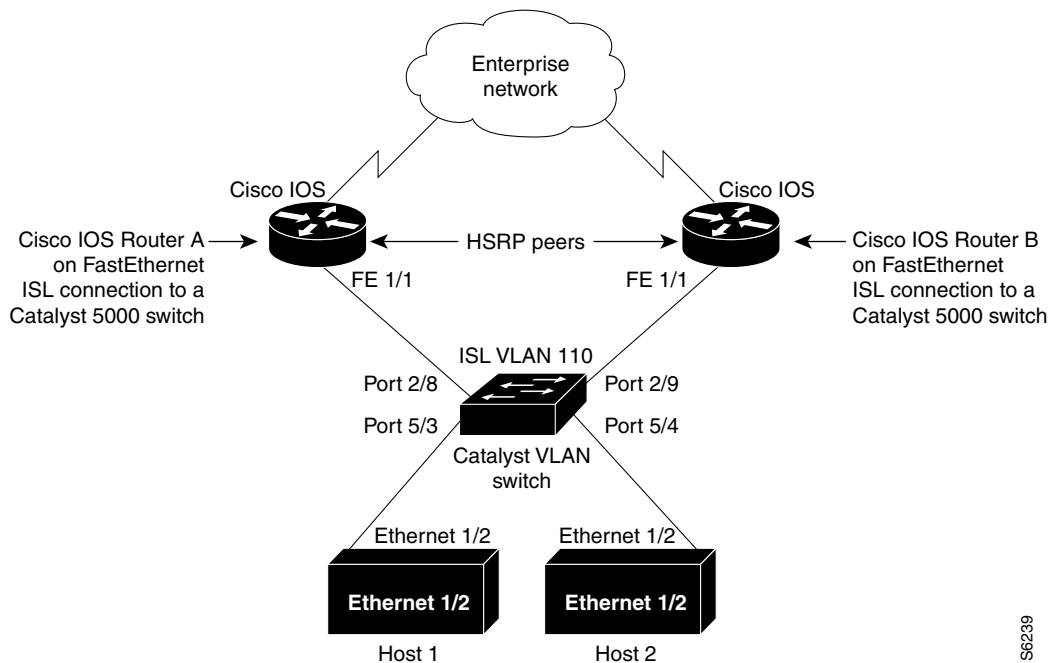
Figure 40 Hot Standby Router Protocol Sample Configuration
