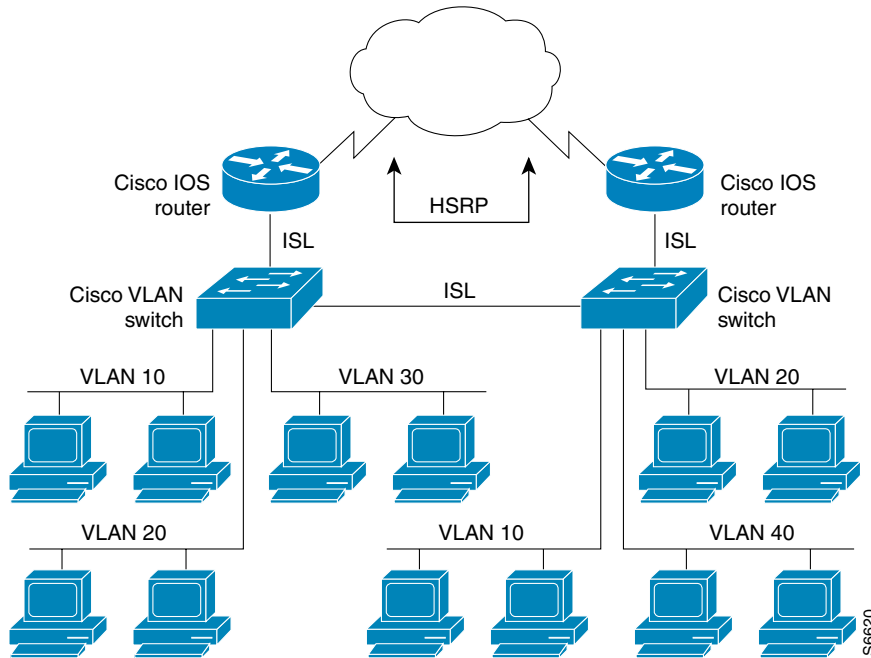
Figure 37 Hot Standby Router Protocol in VLAN Configurations
