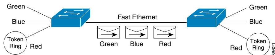
Figure 36 VLAN Packets Traversing the Shared Backbone
