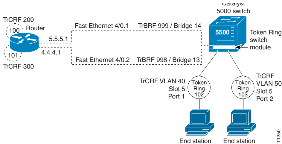
Figure 41 IP Routing with RIF between TrBRF VLANs
