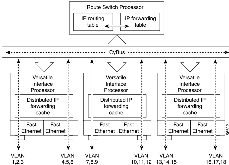
Figure 38 Cisco 7500 Distributed Architecture
