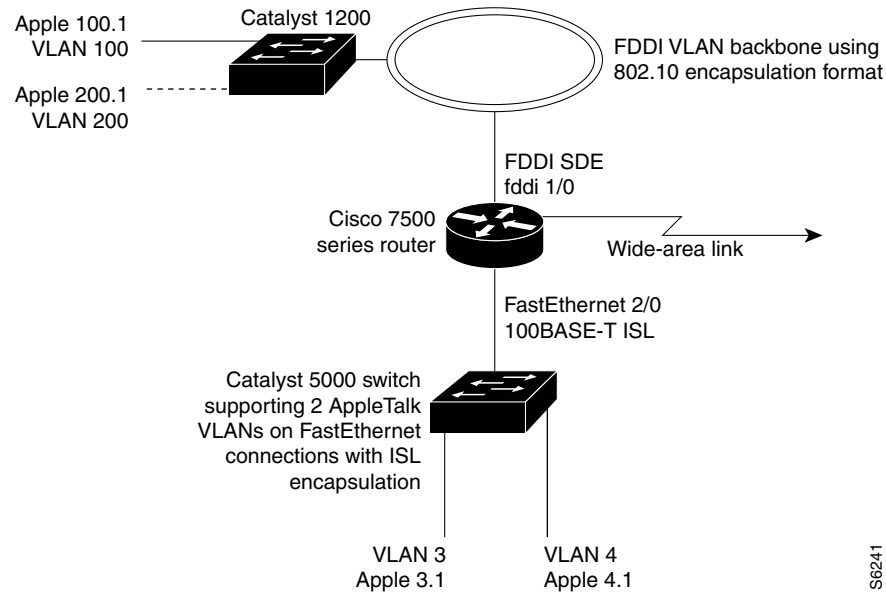
Figure 39 Routing AppleTalk over VLAN Encapsulations
