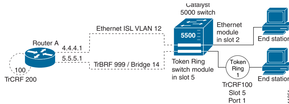
Figure 42 IP Routing Between a TRISL VLAN and an Ethernet ISL VLAN
