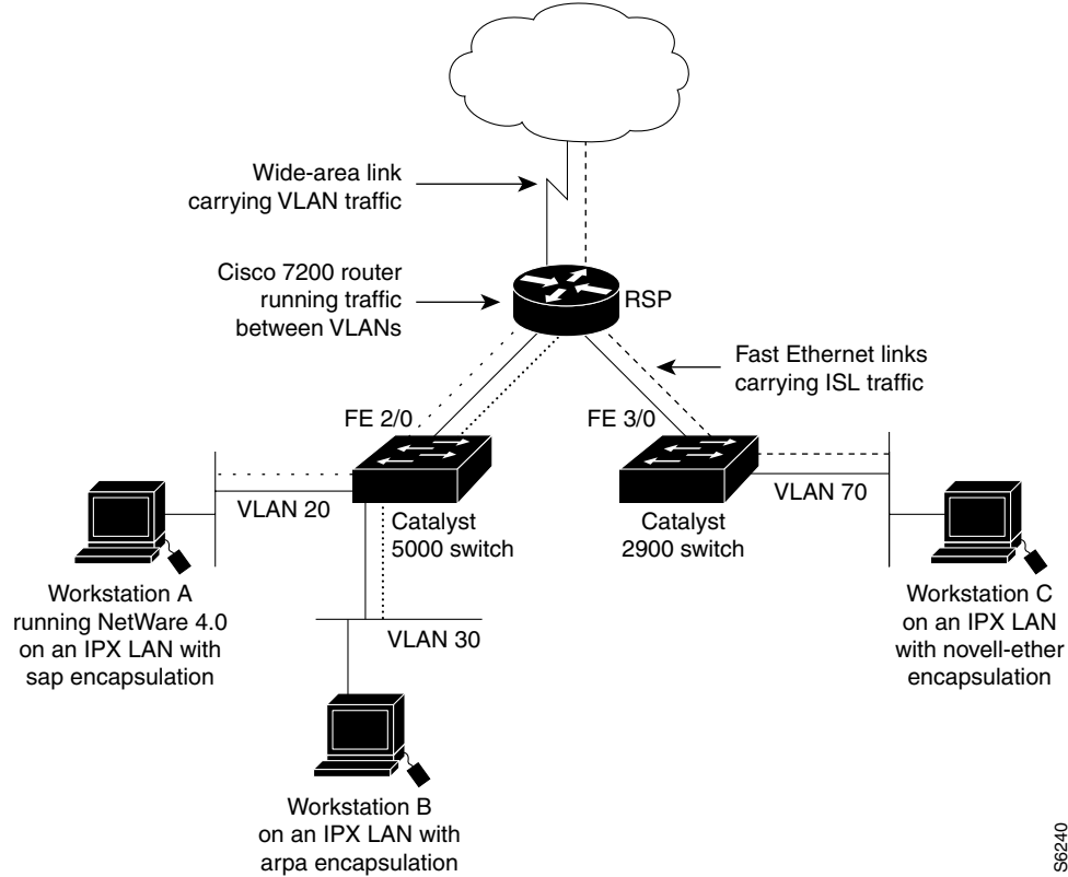
Figure 43 Configurable IPX Encapsulations Routed over ISL in VLAN Configurations
