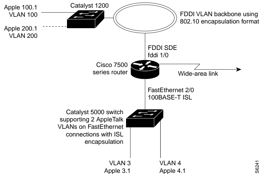
Figure 46 Routing AppleTalk over VLAN encapsulations
