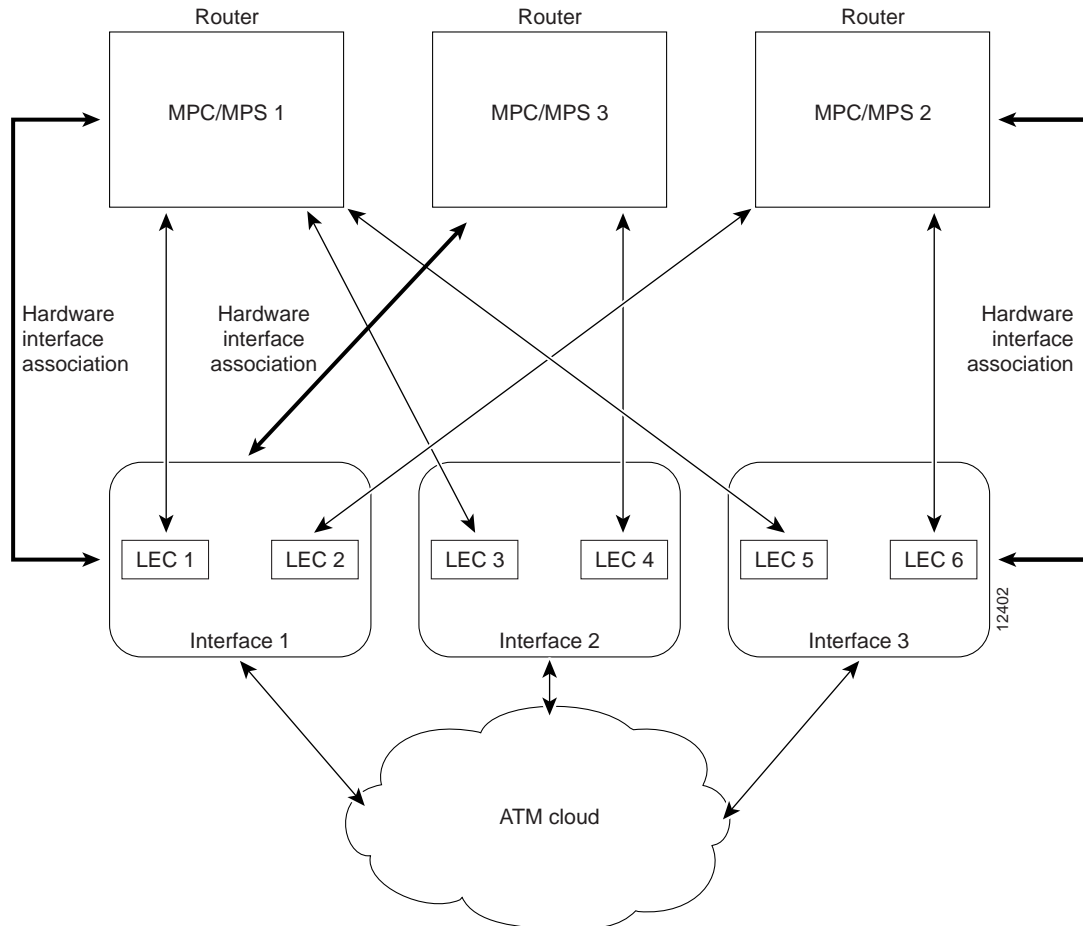
Figure 57 MPC-LEC and MPS-LEC Relationships
