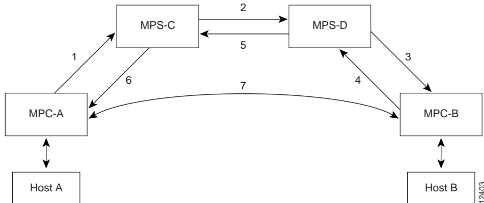
Figure 56 MPOA Message Flow Between MPCs and MPSs
