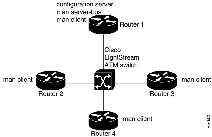
Figure 48 Single Emulated LAN Configured on Several Routers
