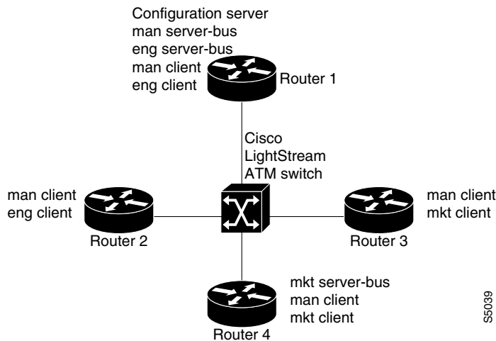
Figure 49 Multiple Emulated LANs Configured on Several Routers
