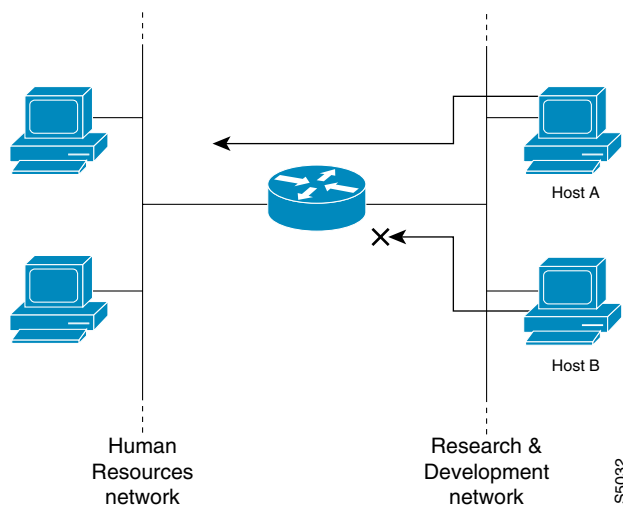
Figure 8 Using Traffic Filters to Prevent Traffic from Being Routed to a Network
