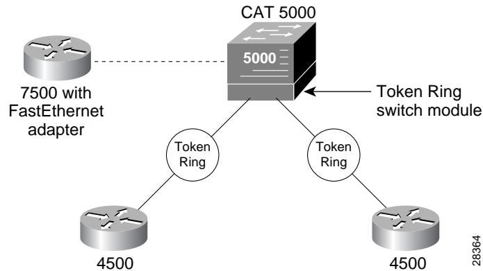
Figure 68 Sample Configuration of TRISL with Fast EtherChannel
