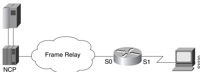
Figure 192 SDLC-Attached SNA Devices
