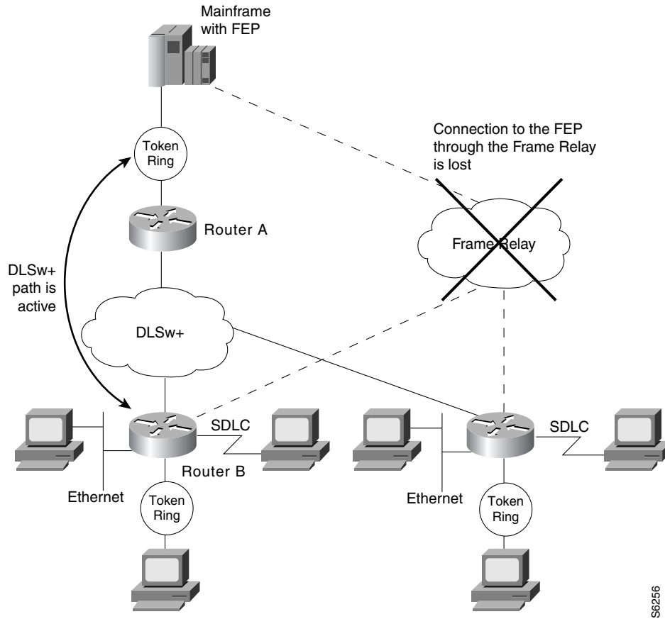
Figure 188 FRAS Dial Backup over DLSw+ when Frame Relay Unavailable
