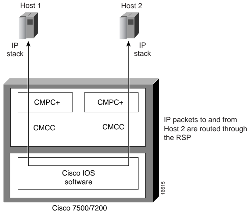
Figure 281 IP Communication Between IBM Hosts Using Different CMCC Adapters
