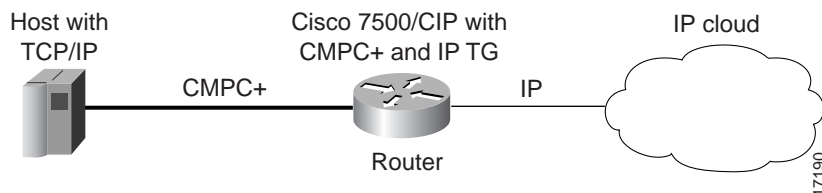
Figure 290 CMPC+ IP with TCP/IP
