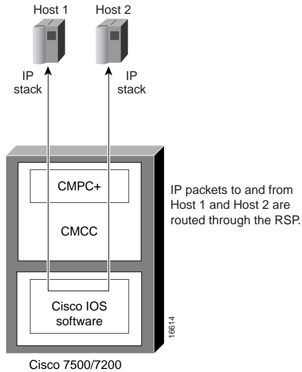
Figure 280 IP Communication Between IBM Hosts Through the Same CMCC
