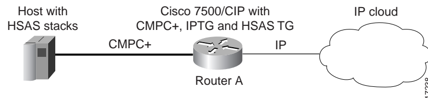
Figure 293 CMPC+ with Split TG
