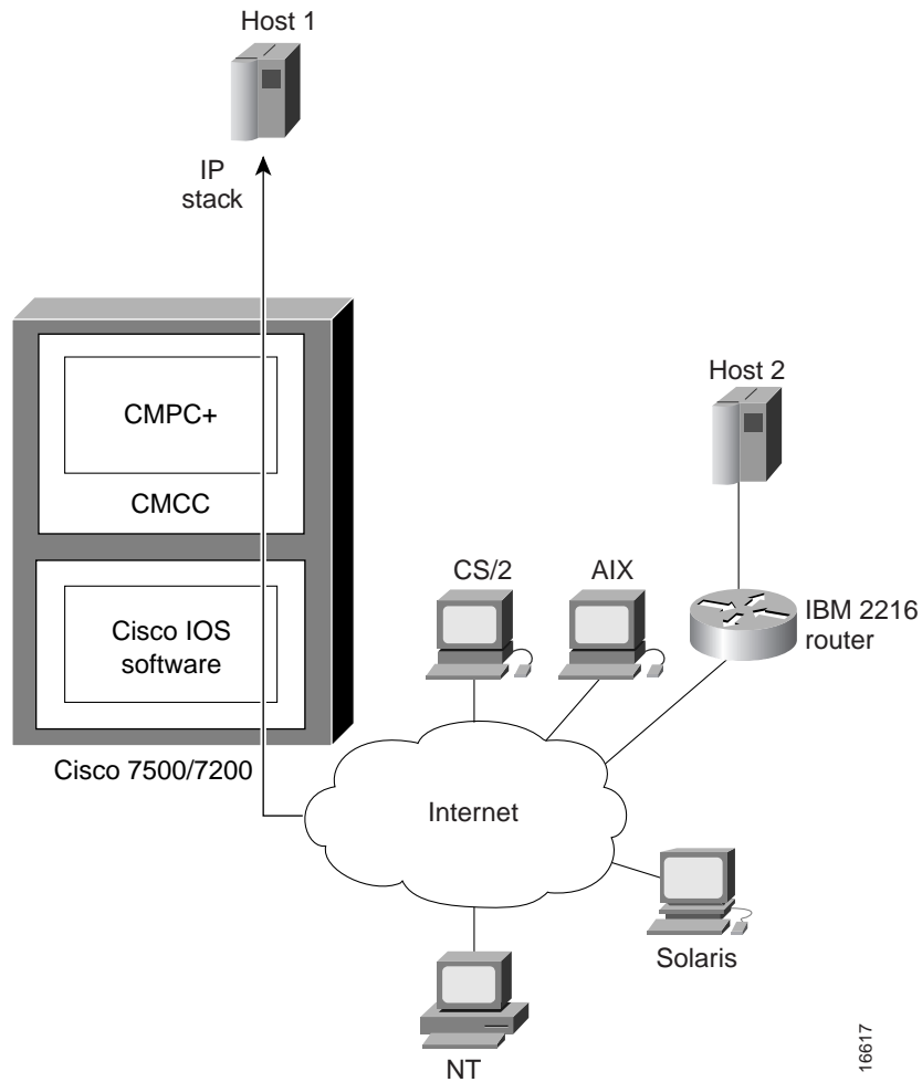
Figure 283 IP Communication from a Host to IP Nodes
