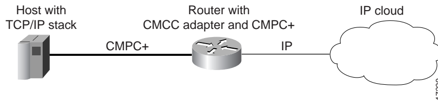
Figure 278 MVS Host with TCP/IP Stack and Cisco Router with CMPC+
