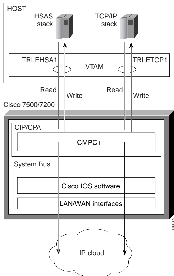
Figure 279 CMPC+ IP Structure
