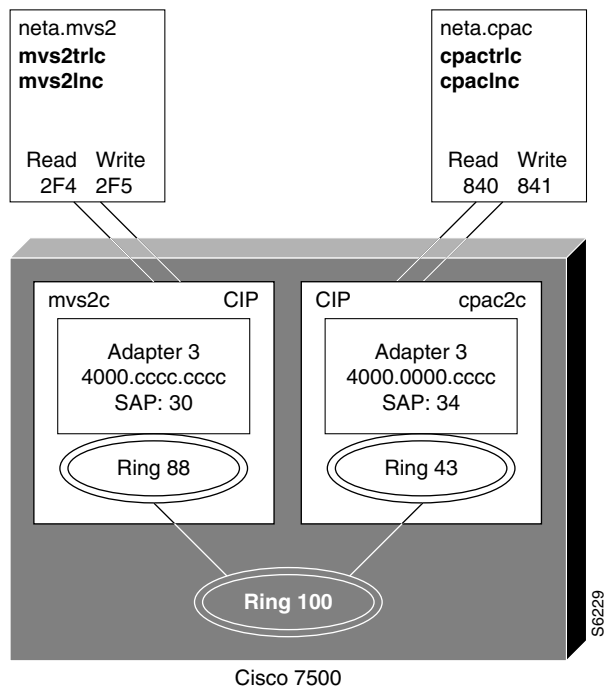
Figure 275 Parameters for VTAM-to-VTAM Connection
