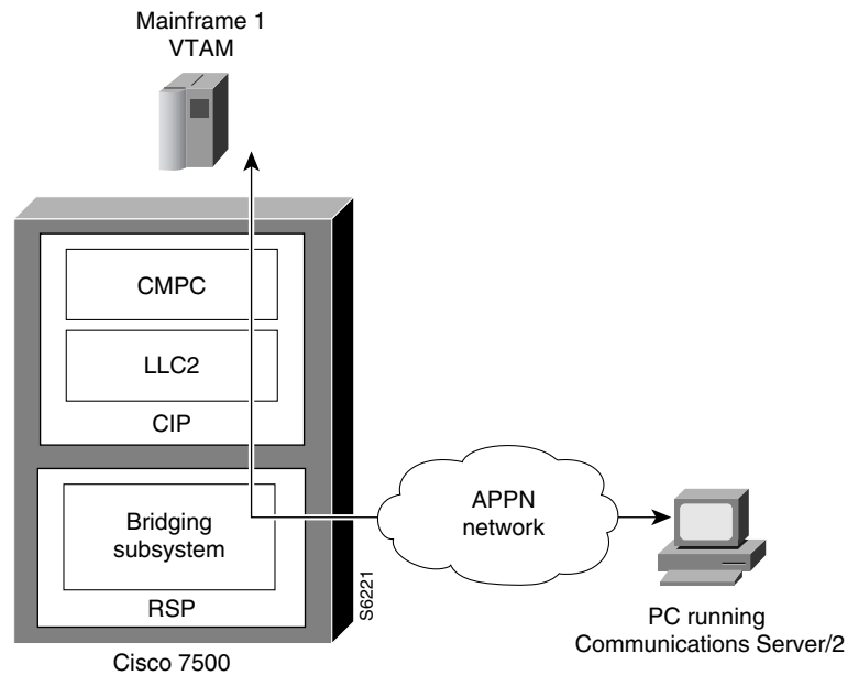
Figure 270 Topology for VTAM-to-Remote PC with Communications Server/2
