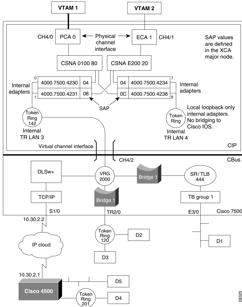
Figure 268 CIP CSNA Source-Route Translational Bridging Configuration
