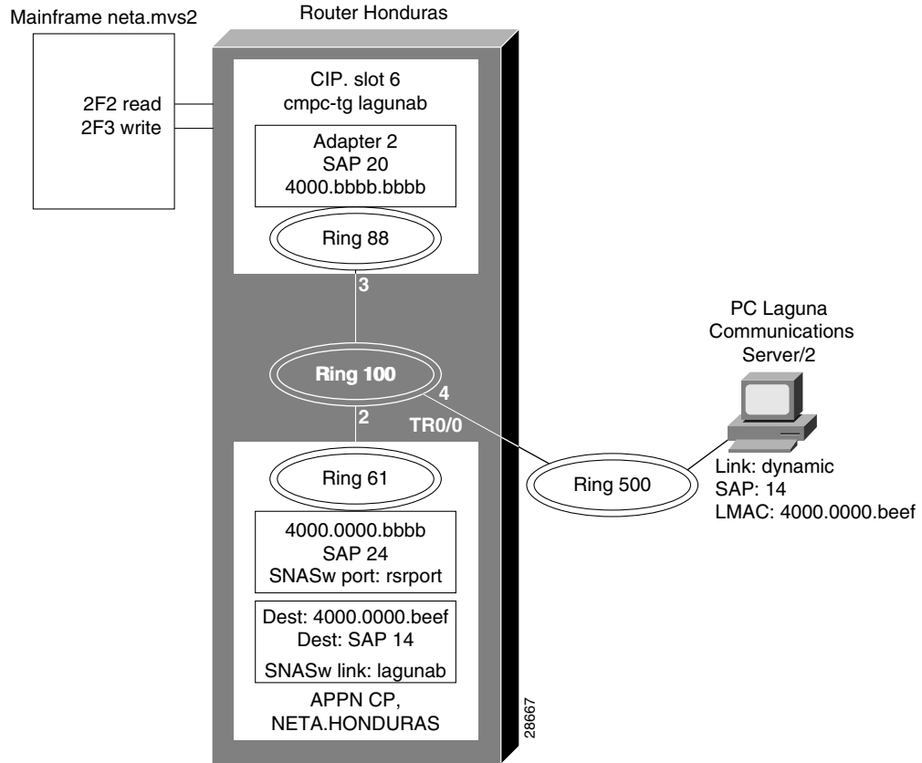
Figure 273 Parameters for VTAM-to-SNASw Connection on the CIP
