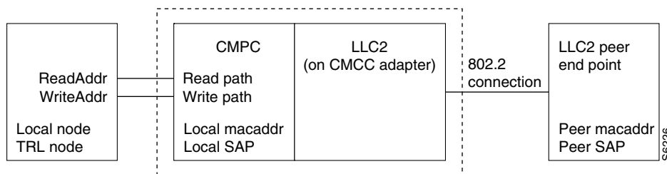
Figure 261 Logical View of CMPC Link
