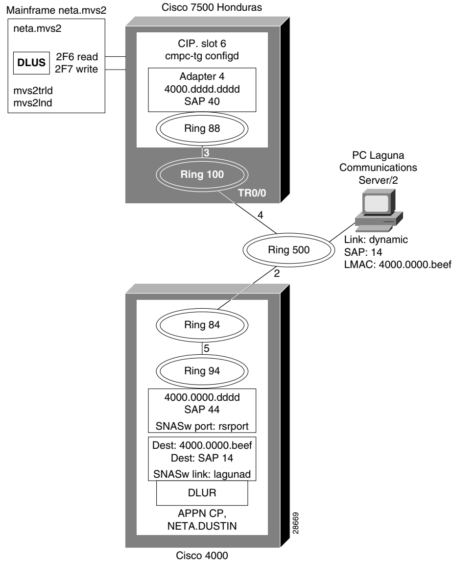
Figure 277 Parameters for VTAM-to-SNASw on a Remote Router with DLUR Connection
