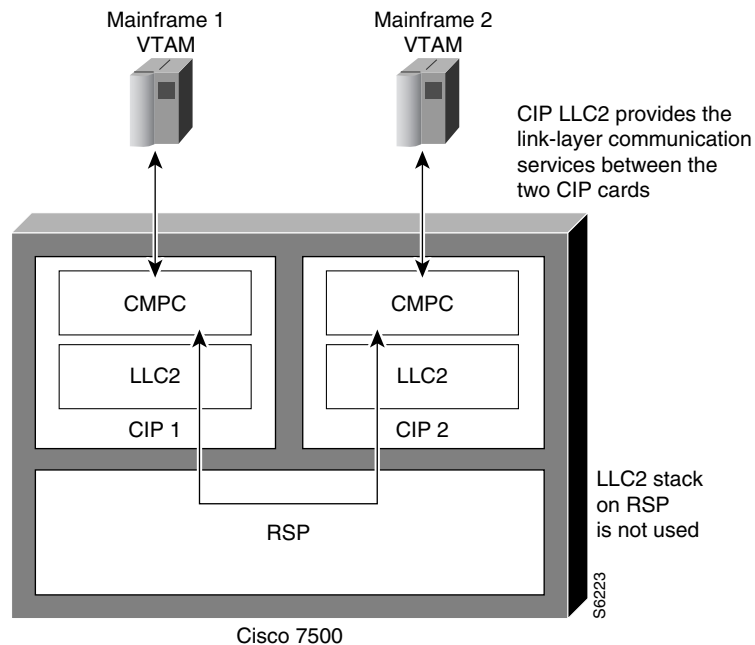
Figure 274 Topology for VTAM-to-VTAM Connection
