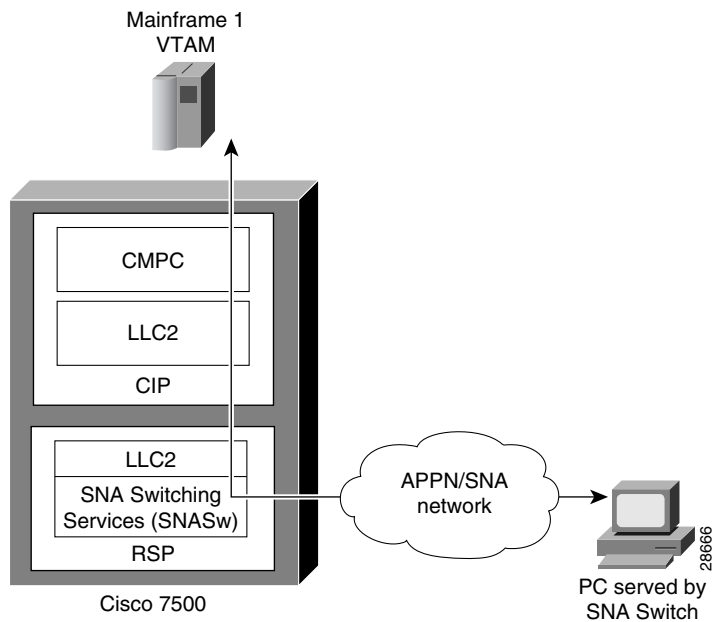
Figure 272 Topology for VTAM-to-SNASw Connection on the CIP
