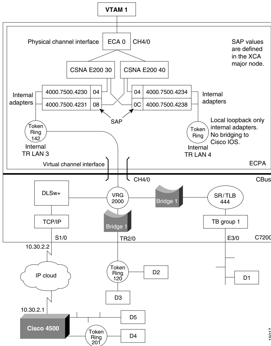
Figure 269 ECPA CSNA Source-Route Translational Bridging Configuration
