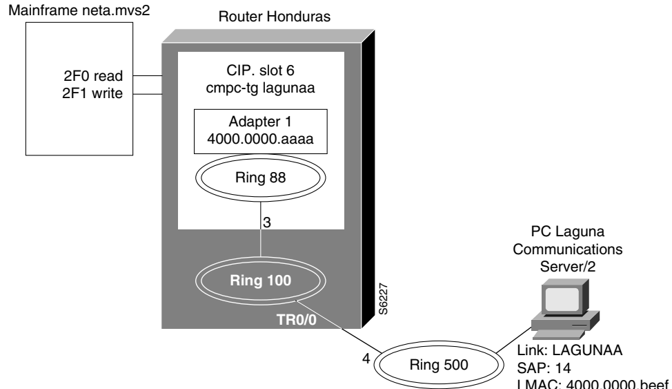
Figure 271 Parameters for VTAM-to-Remote PC with Communications Server/2
