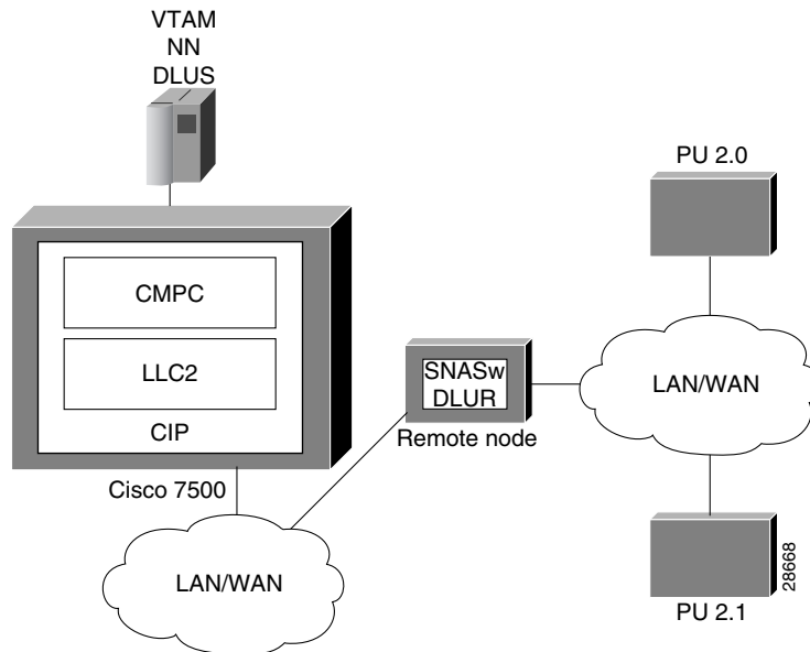
Figure 276 Topology for VTAM-to-SNASw on a Remote Router with DLUR Connection
