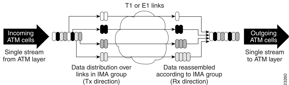
Figure 1 Inverse Multiplexing and Demultiplexing
