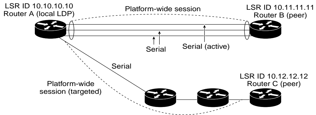
Figure 5 Hello Adjacency
