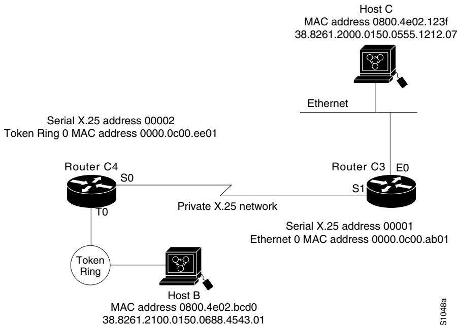
Figure 27 Example Network Topology for Switching CMNS over a Leased Line
