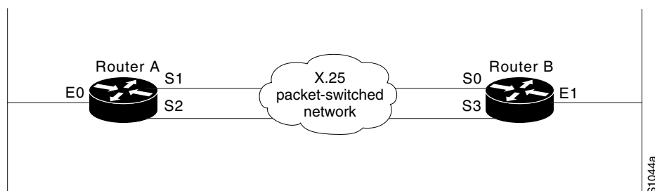
Figure 28 Parallel Serial Lines to an X.25 Network
