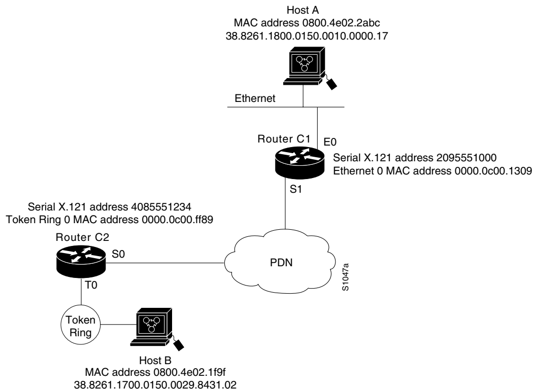
Figure 26 Example Network Topology for Switching CMNS over a PDN
