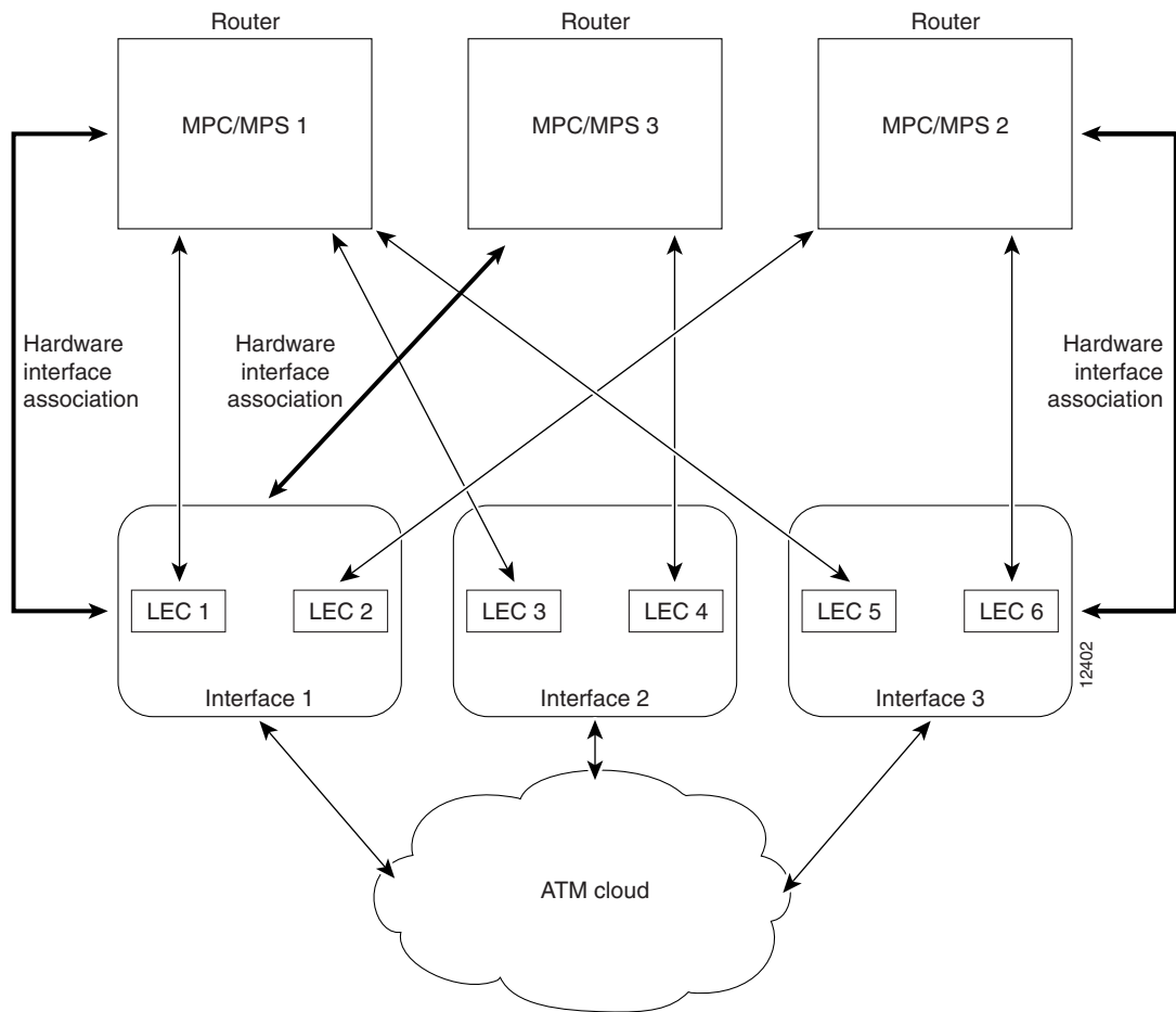
Figure 38 MPC-LEC and MPS-LEC Relationships
