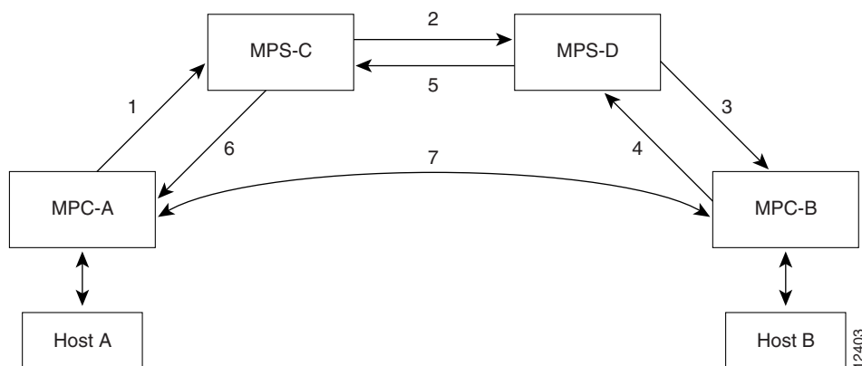
Figure 37 MPOA Message Flow Between MPCs and MPSs
