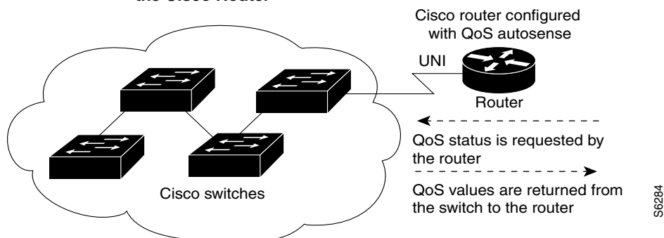
Figure 11 Enhanced Local Management Interface—Sent between the Cisco Switch and the Cisco Router
