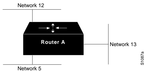
Figure 28 Helper Addresses
