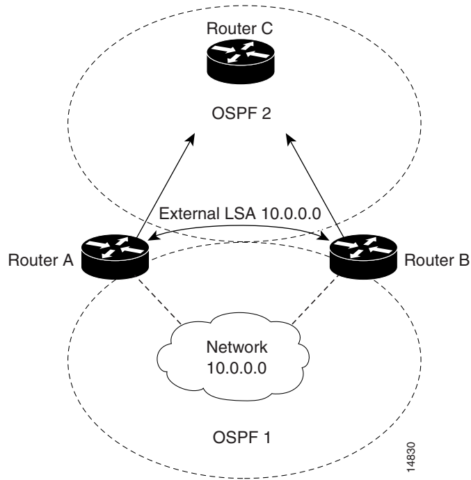
Figure 26 OSPF Administrative Distance
