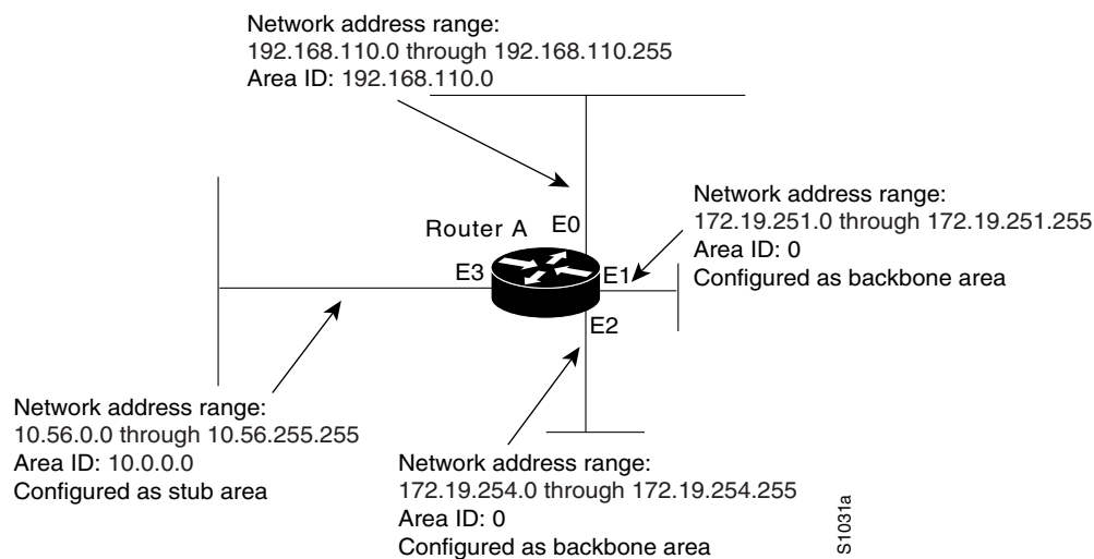
Figure 37 Interface and Area Specifications for OSPF Example Configuration
