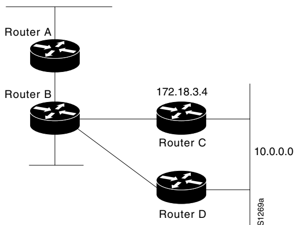
Figure 35 Overriding Static Routes
