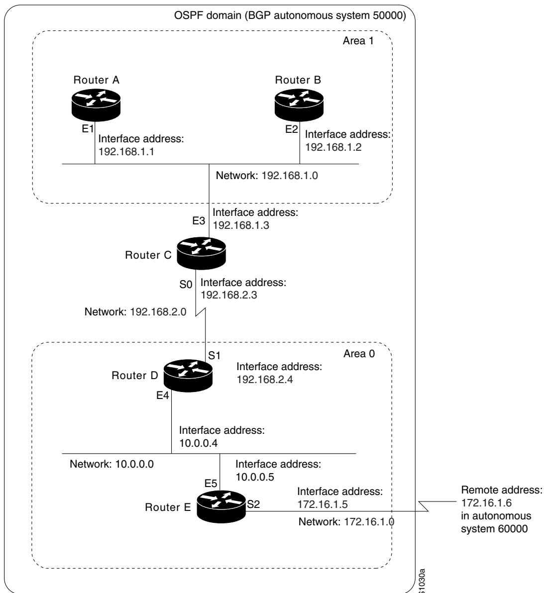
Figure 36 Sample OSPF Autonomous System Network Map
