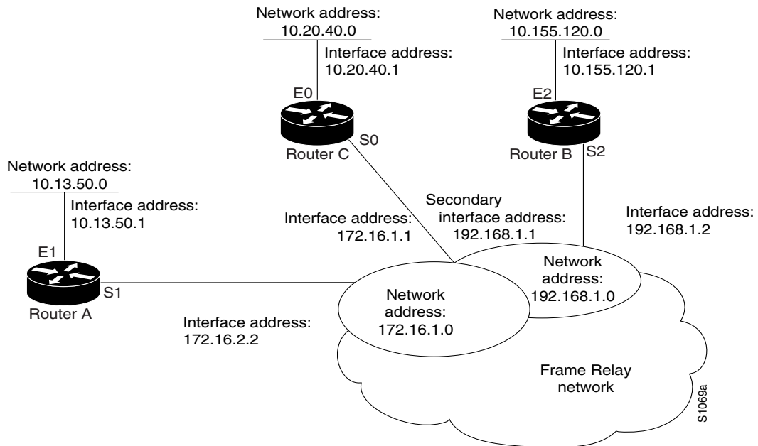
Figure 20 Disabled Split Horizon Example for Frame Relay Network
