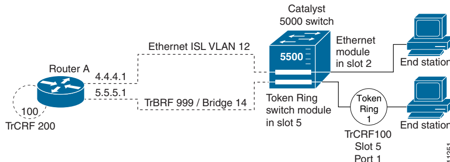
Figure 75 IP Routing Source-Routed Frames between a TRISL VLAN and an Ethernet ISL VLAN
