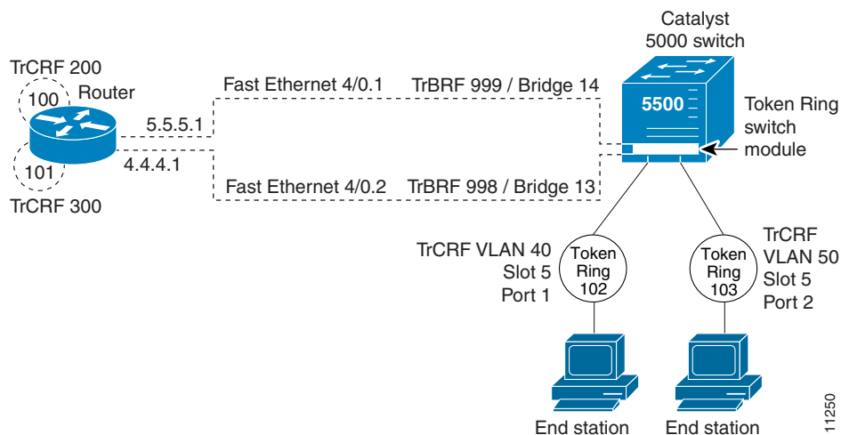
Figure 76 IP Routing Source-Routed Frames between TrBRF VLANs
