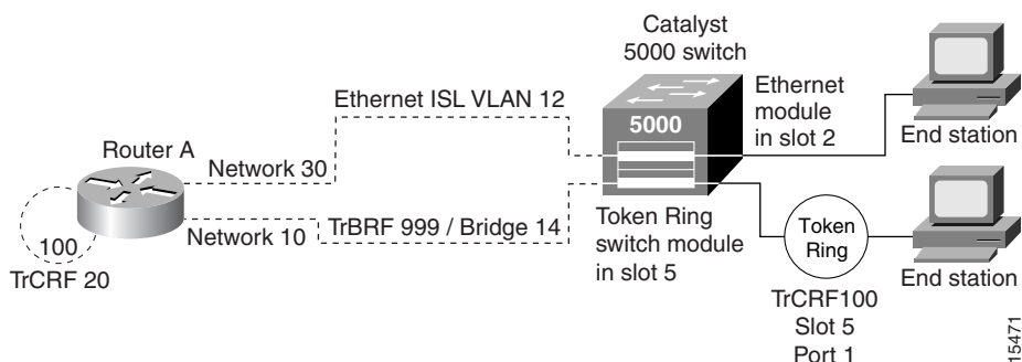
Figure 79 IPX Routing Source-Routed Frames between a TRISL VLAN and an Ethernet ISL VLAN
