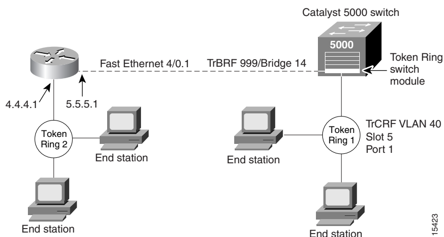
Figure 73 IP Routing between a TRISL VLAN and a Token Ring Interface
