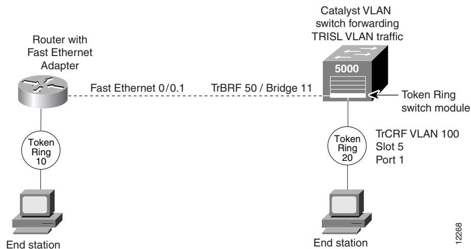
Figure 83 Transparent Bridging between Token Ring and TRISL VLAN
