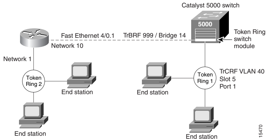
Figure 77 IPX Routing Non-Source-Routed Frames between a TRISL VLAN and a Token Ring Interface Example
