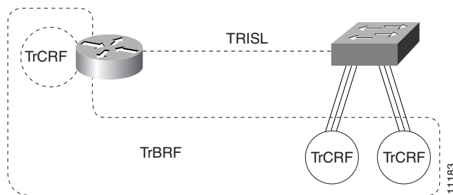
Figure 72 TrCRFs in a TrBRF
