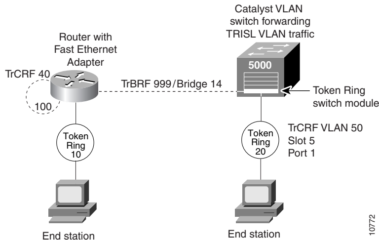
Figure 81 SRB between a Token Ring Interface and TRISL VLAN
