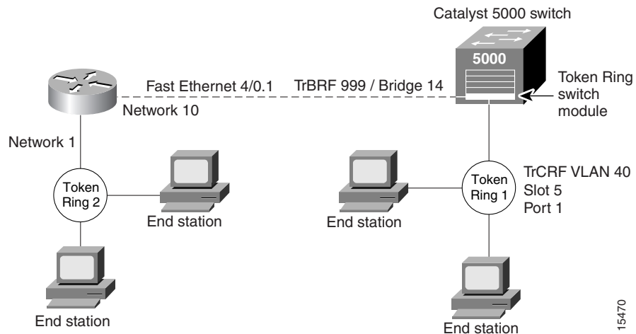
Figure 78 IPX Routing Source-Routed Frames between a TRISL VLAN and a Token Ring Interface
