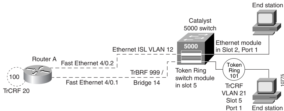
Figure 85 SR/TLB between a TRISL VLAN and an Ethernet ISL VLAN
