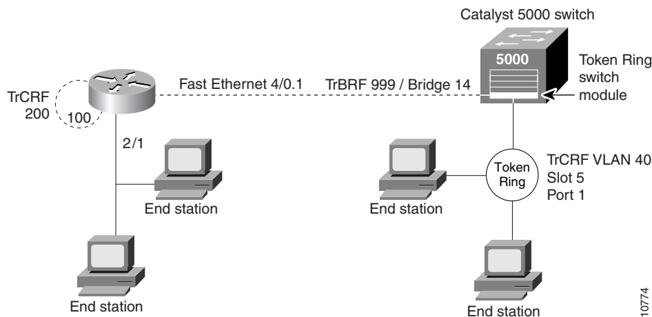
Figure 84 SR/TLB between a TRISL VLAN and an Ethernet Interface
