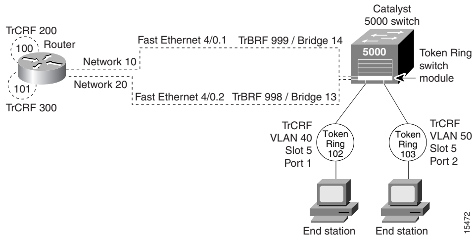
Figure 80 IPX Routing Source-Routed Frames between TRISL VLANs
