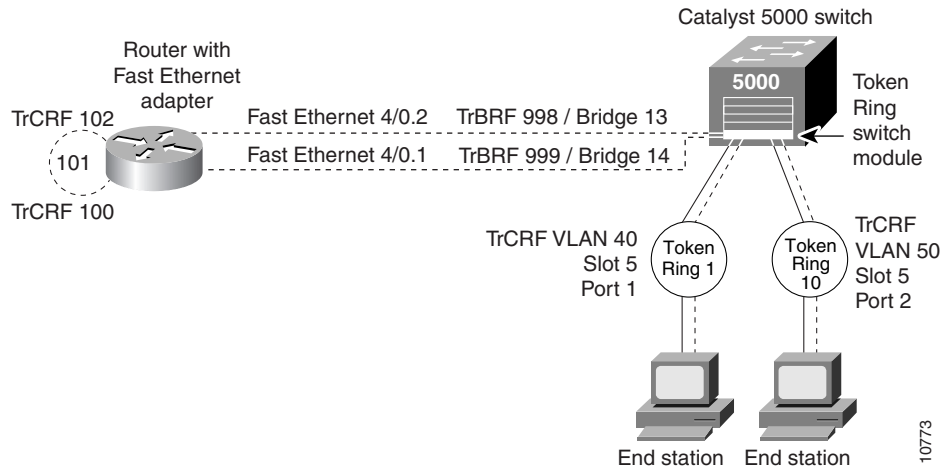
Figure 82 SRB between TRISL VLANs
