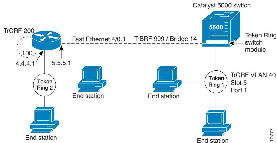
Figure 74 Routing Source-Routed Frames between a TRISL VLAN and a Token Ring Interface
