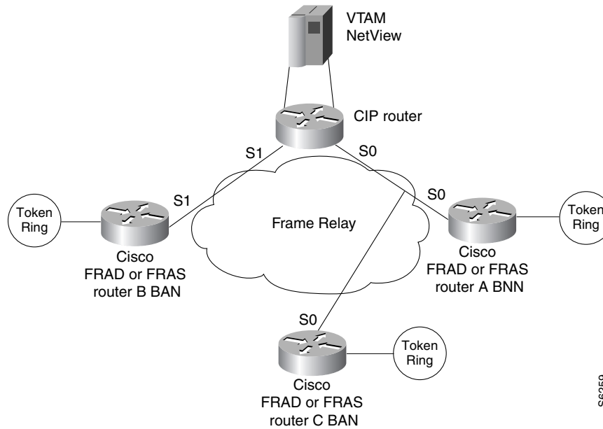
Figure 146 FRAS Host CIP Connection to VTAM
