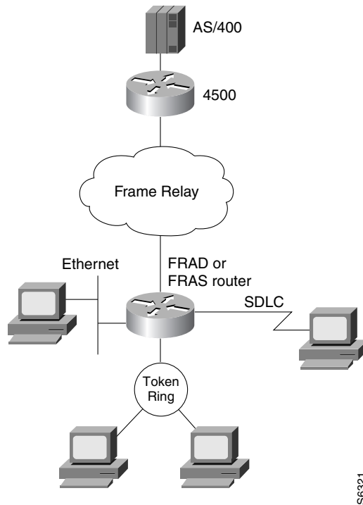
Figure 147 FRAS Host Ethernet Connection to AS/400
