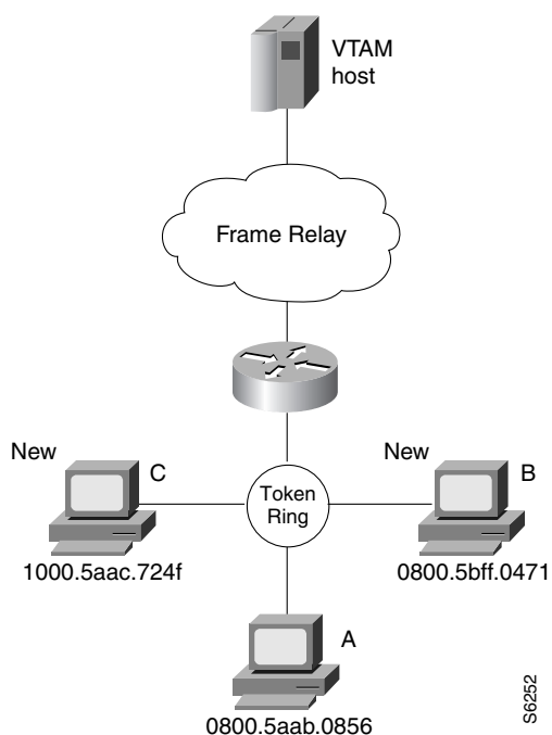
Figure 144 FRAS BNN Configuration
