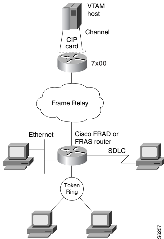
Figure 138 Cisco FRAD Access to a Mainframe through a Cisco 7500
