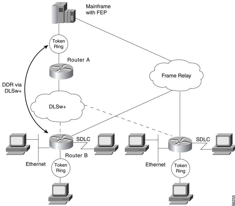
Figure 136 FRAS Dial Backup over DLSw+
