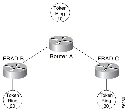
Figure 145 FRAD Using SRB over Frame Relay to Connect to a Cisco Router
