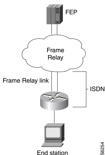
Figure 135 FRAS DLCI Backup over ISDN
