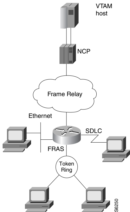
Figure 142 FRAS BNN Topology
