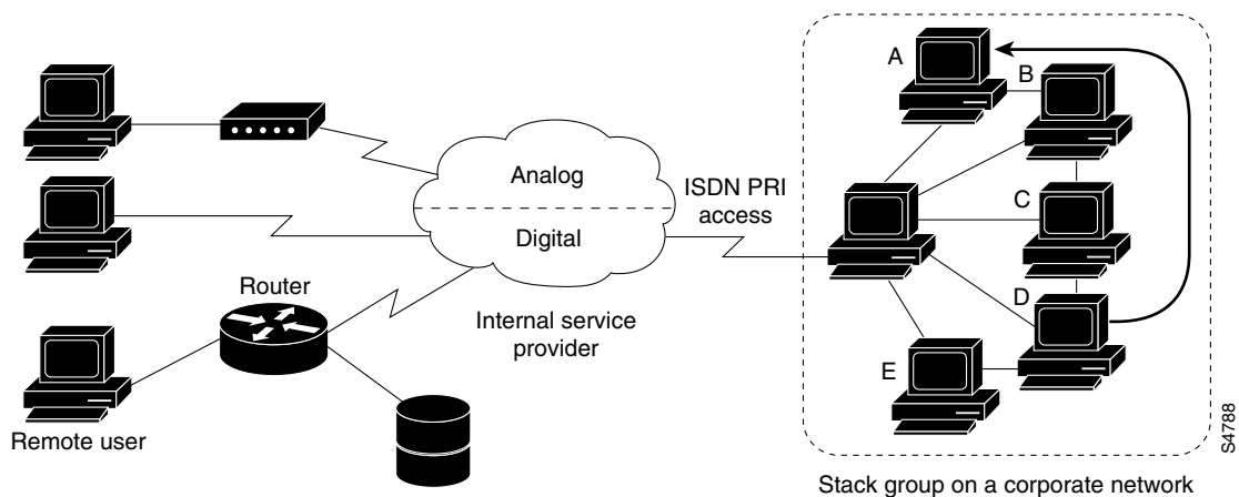
Figure 306 Typical Multichassis Multilink PPP Scenario
