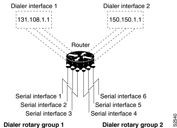
Figure 294 Sample Dialer Interface Configuration
