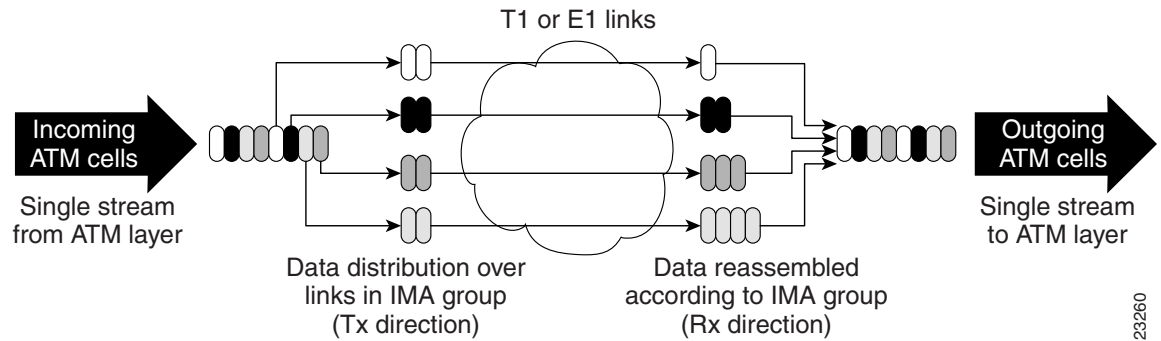
Figure 2 Inverse Multiplexing and Demultiplexing
