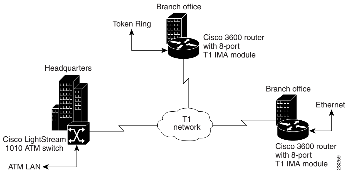
Figure 1 LAN-to-WAN Application Connectivity with T1 and IMA
