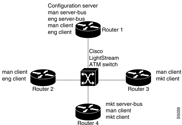
Figure 20 Multiple Emulated LANs
