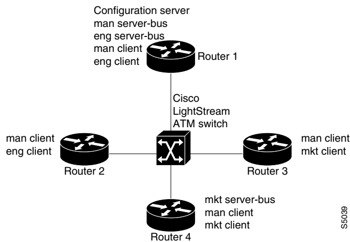
Figure 21 Multiple Emulated LANs with Restricted Membership
