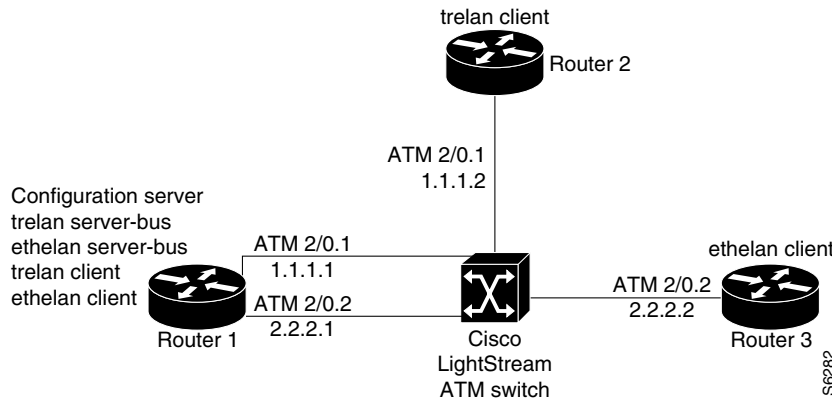
Figure 24 Routing between Token Ring and Ethernet Emulated LANs
