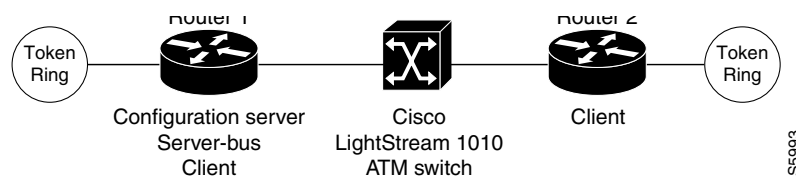
Figure 22 2-Port Source-Route Bridging TR-LANE
