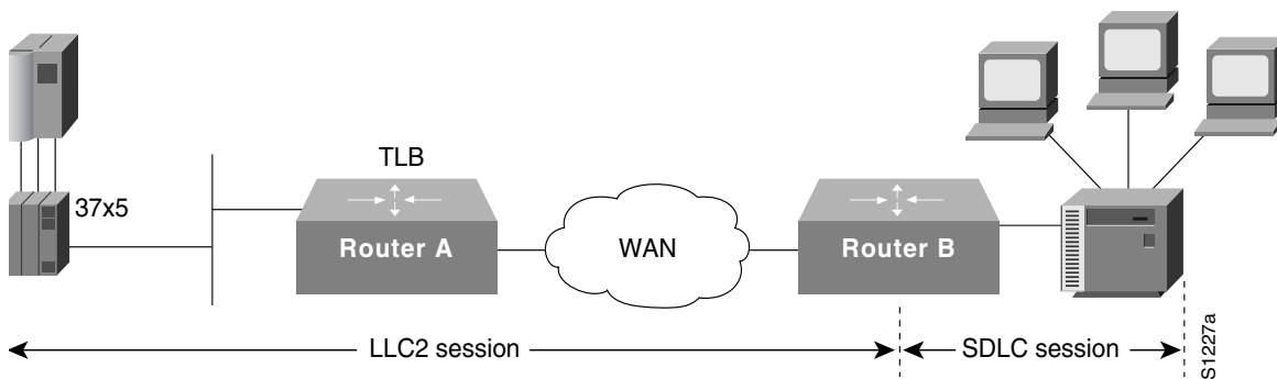
Figure 108 SDLLC with Ethernet and Translational Bridging
