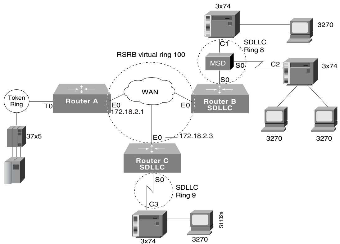
Figure 112 SDLLC with RSRB with Multiple 3x74s
