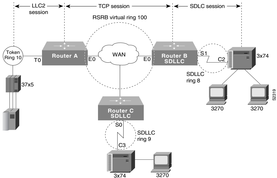
Figure 113 SDLLC with RSRB and Local Acknowledgment
