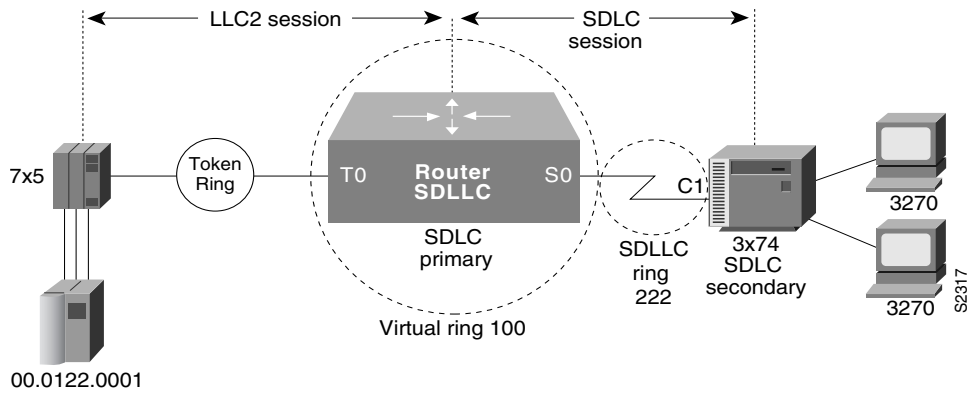
Figure 109 SDLLC Communication between a 37x5 and a 3x74 Connected to the Same Router (Direct Connection)
