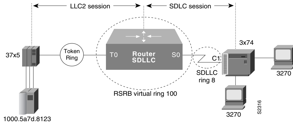
Figure 110 SDLLC with Single Router Using RSRB
