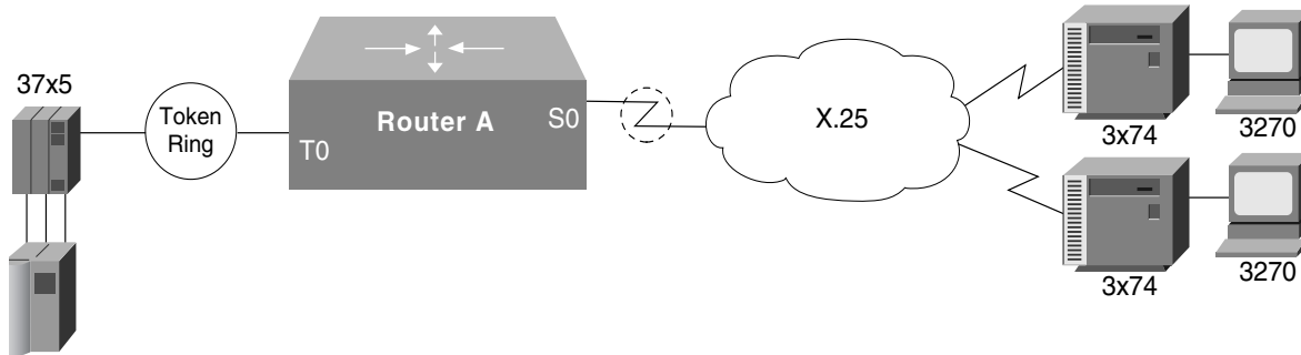
Figure 114 QLLC Conversion between a Single 37x5 and Multiple 3x74s
