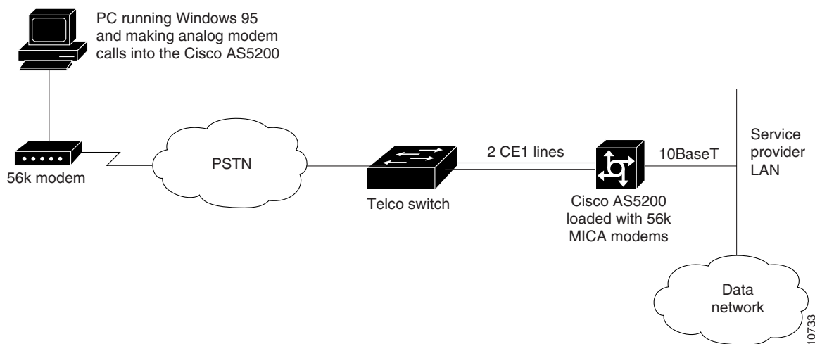
Figure 1 Service Provider using E1 R1 Signaling with a Cisco AS5200
