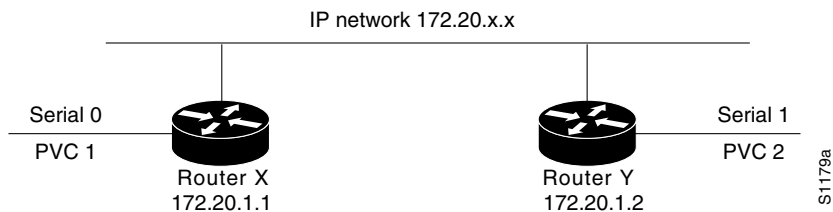
Figure 48 X.25 Tunneling Connection
