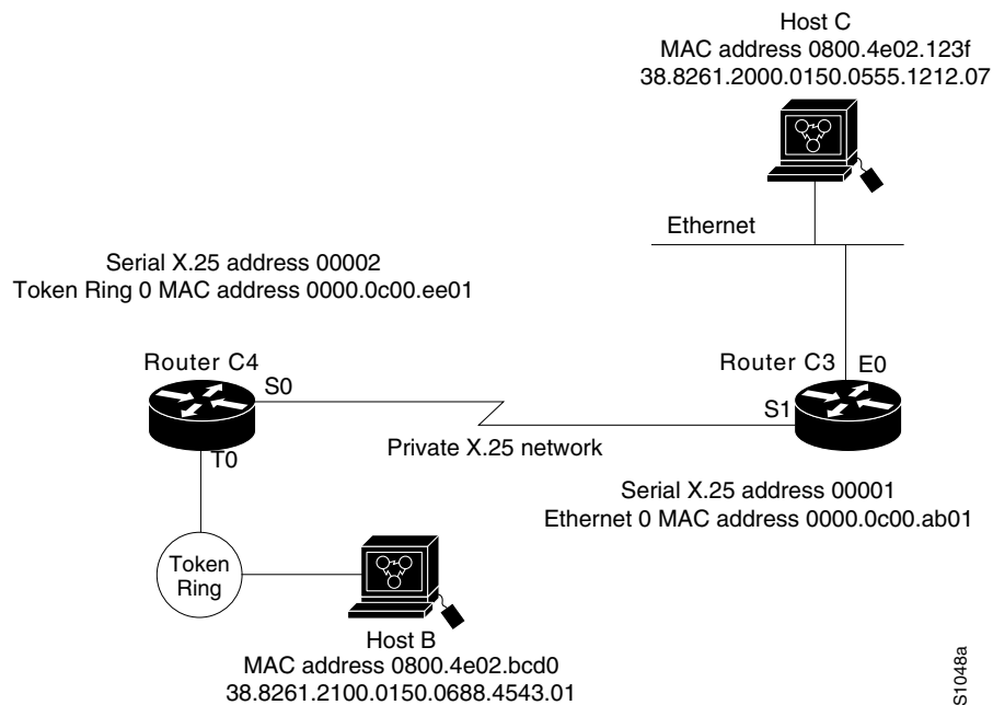
Figure 51 Example Network Topology for Switching CMNS over a Leased Line
