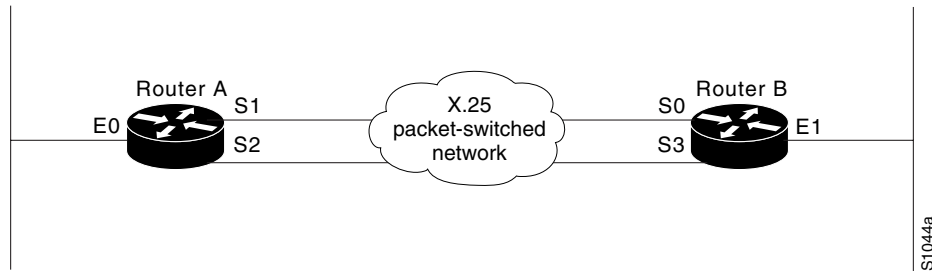
Figure 52 Parallel Serial Lines to an X.25 Network
