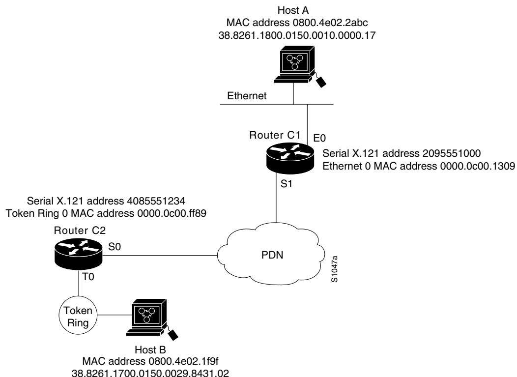
Figure 50 Example Network Topology for Switching CMNS over a PDN
